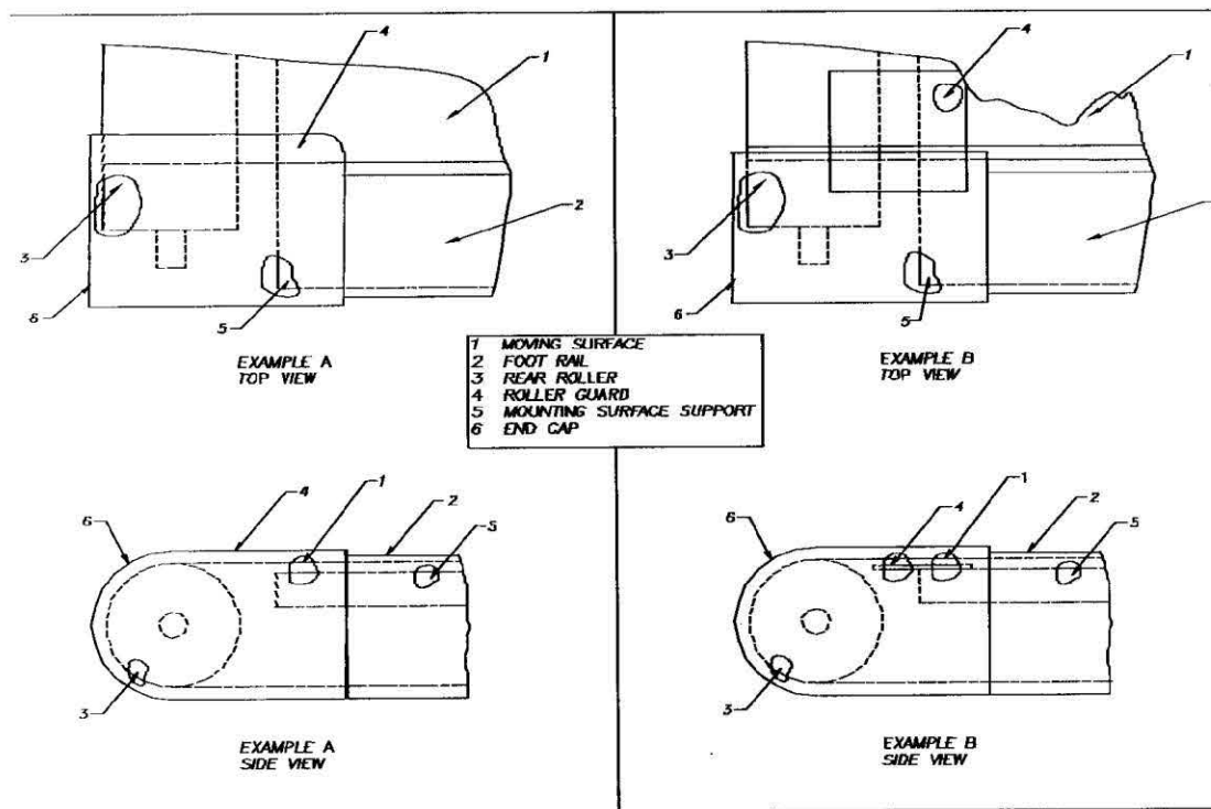
FIG. 2 Examples of Rear Roller Guarding
