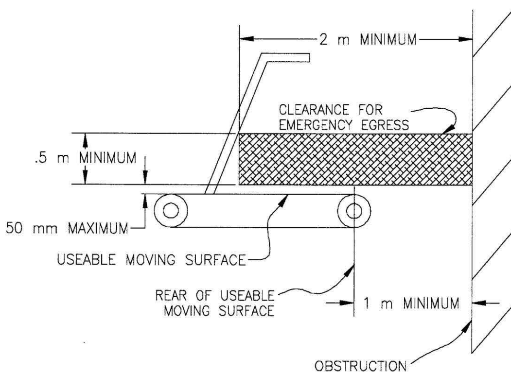
FIG. 4 Minimum Clearance for Emergency Dismount
