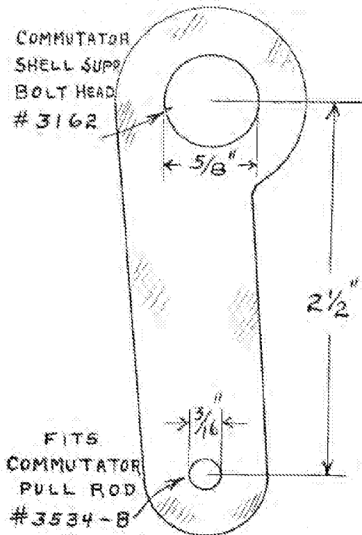
Full Size Gauge for Adjusting Timer.
