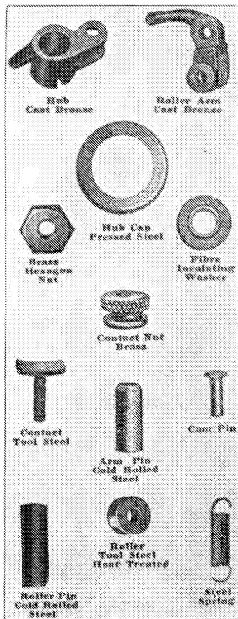
Timer Components.
