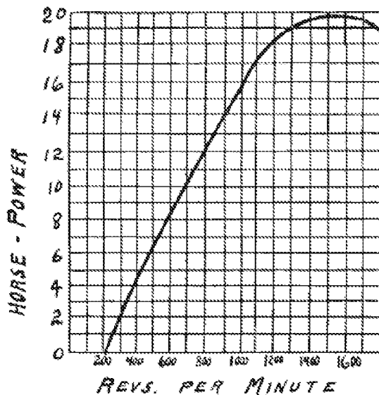
POWER CURVE OF FORD
