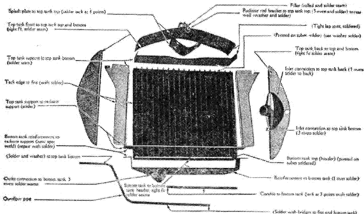
Present Type of Ford Radiator.
