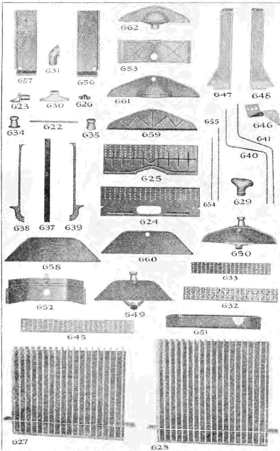
Radiator Parts.
