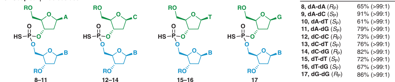
Fig. 2. Formalisms for the use of \psi reagents in dinucleotide synthesis. (A) Stereochemical assignments. (B) Loading of nucleoside monomers. (C) Coupling to produce stereopure PS dinucleotides. R, TBDPS ( tert -butyldiphenylsilyl). Loading:
