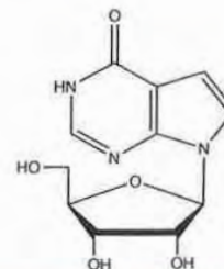
RP-2314 7-deaza-Inosine
