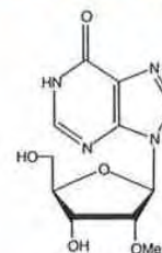
RP-1906 2'-(O-Methyl)-Inosine
