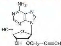
RP-3401 2'-O-propargyl-Adenosine
