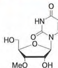
RP-2904 3'-(O-Methyl)-Uridine
