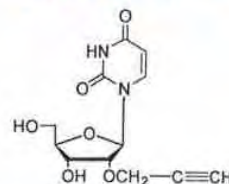
RP-3404 2'-O-propargyl-Uridine
