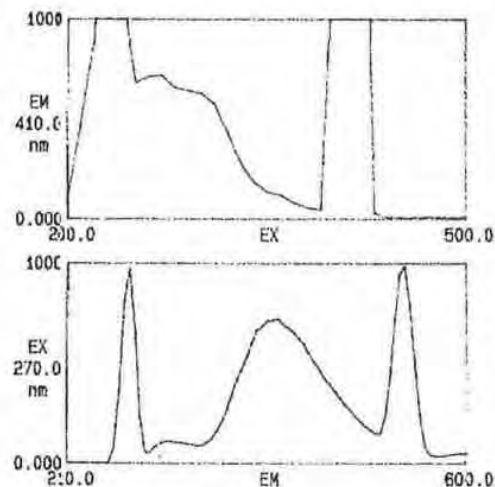
Fig. : A synthetic DNA primer carrying etheno-deoxy-Adenosine units; upper graph showing strong emission at 410 nm, lower graph showing excitation of the same primer at 270 nm.
