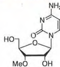
RP-2904 3'-(O-Methyl)-Uridine
