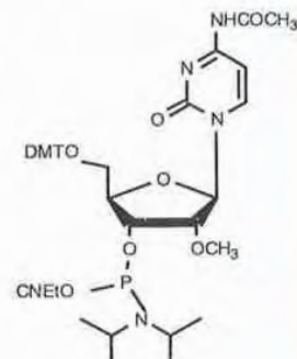
ANP-6756 Ac-Cytidine
