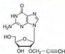
RP-3403 2'-O-propargyl-Guanosine
