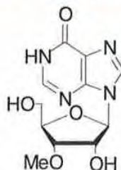
RP-2905 3'-(O-Methyl)-Inosine
