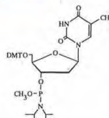
ANP3764 Thymidine
