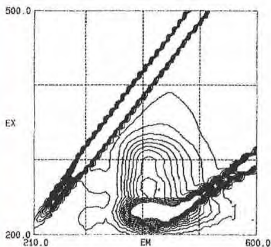
Fig. : DMT-etheno ribo Adenosine three dimensional contour plot of strong emission at 445 nm with excitation at 350 nm.
