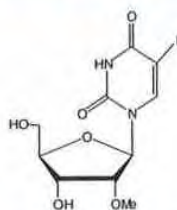
RP-1905 5-Iodo-2'-(O-Methyl)-Uridine
