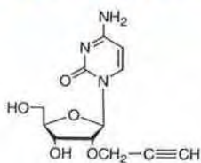
RP-3402 2'-O-propargyl-Cytidine
