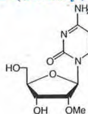
RP-1902 2'-(O-Methyl)-Cytidine
