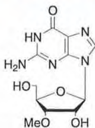
RP-2903 3'-(O-Methyl)-Guanosine
