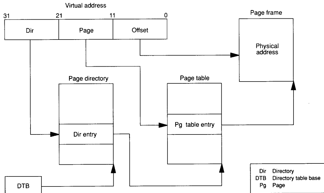
Figure 4. Virtual-to-physical address translation.
