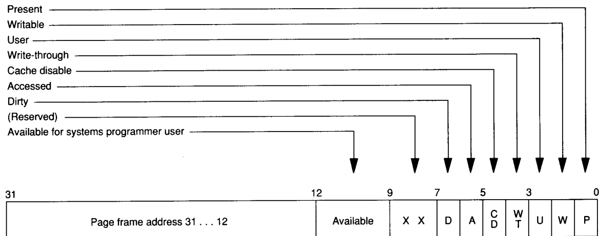
Figure 5. Format of a page table entry. (X indicates Intel reserved; do not use.)
