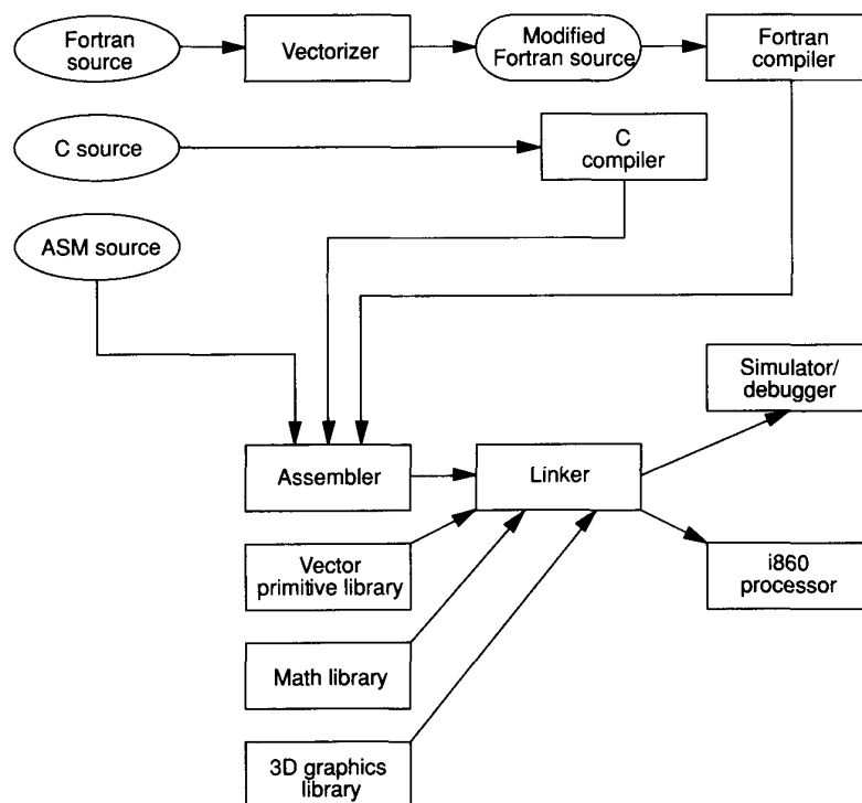
Figure 12. Software development environment supporting the i860.
