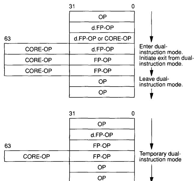
Figure 8. Dual-instruction-mode transitions.
