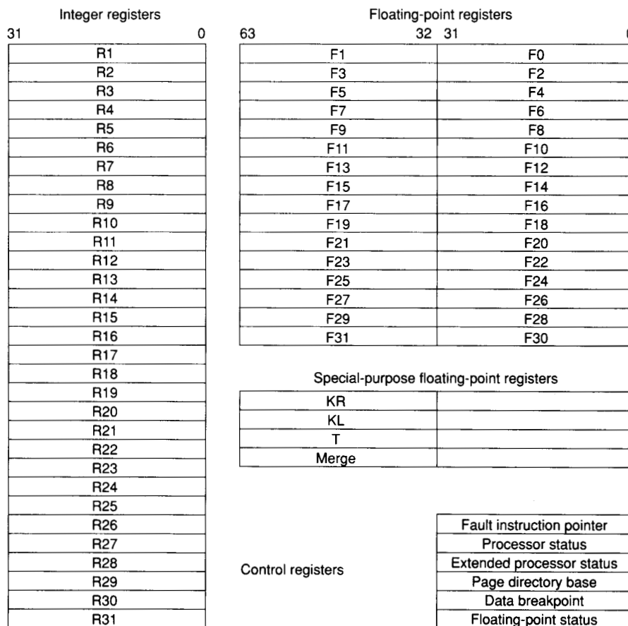
Figure 3. Register set.
