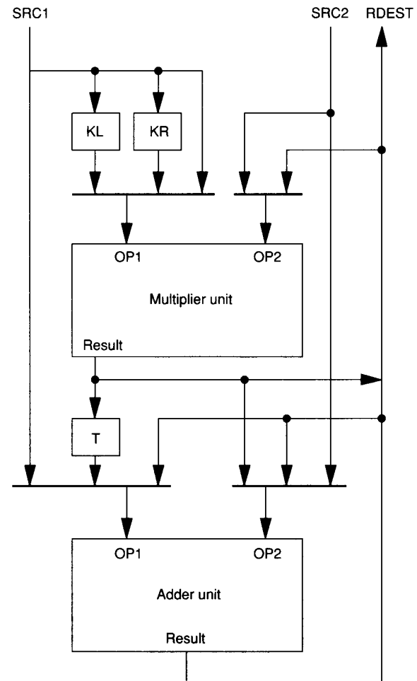
Figure 7. Dual-operation data paths.
