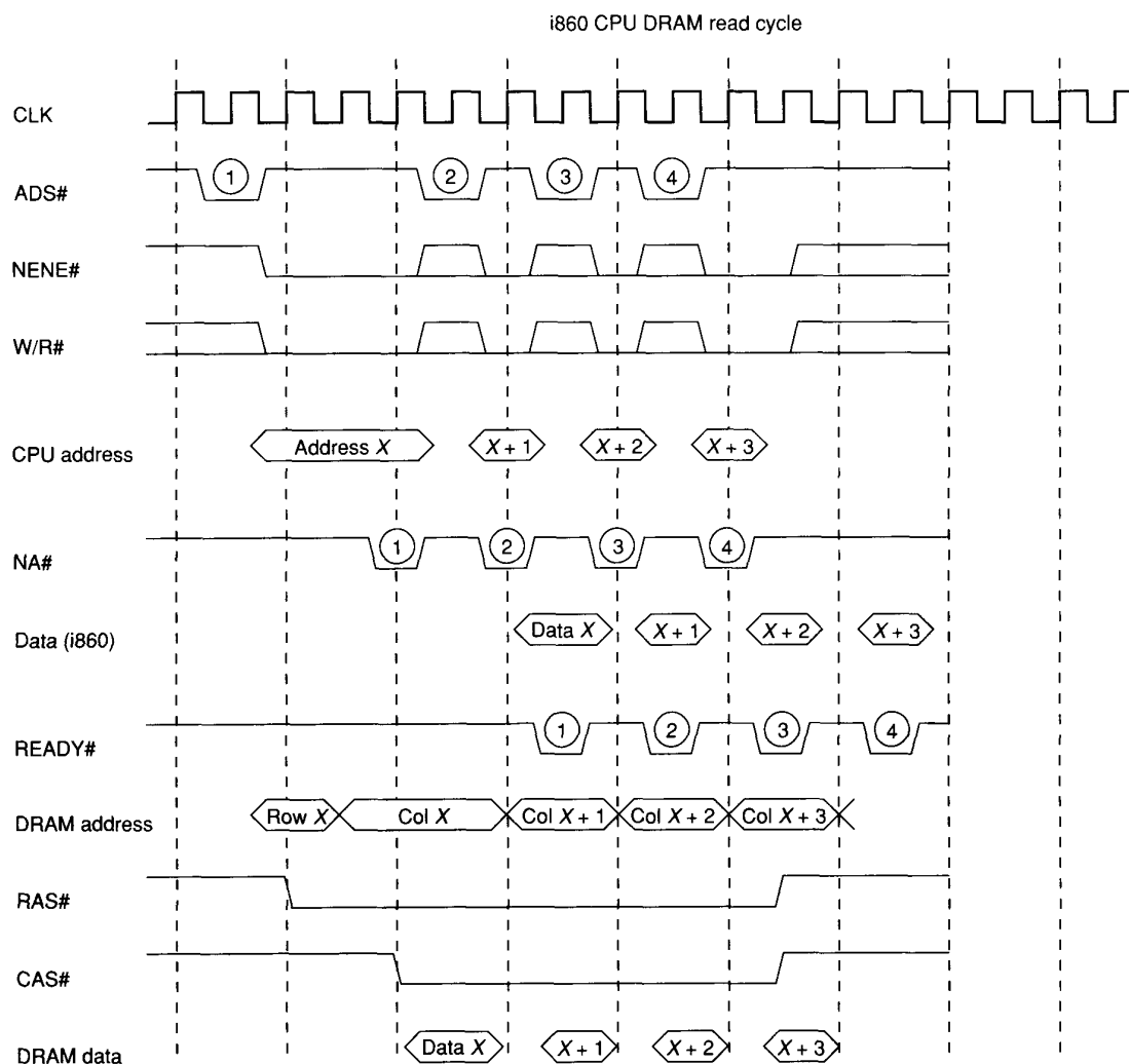
Figure 10. The CPU performs four read cycles to fill a cache line.
