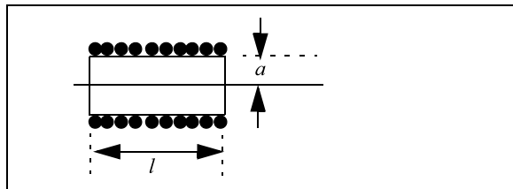
FIGURE 7: A CIRCULAR COIL WITH SINGLE TURN
