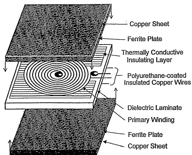
FIG.3 (PRIOR ART)
