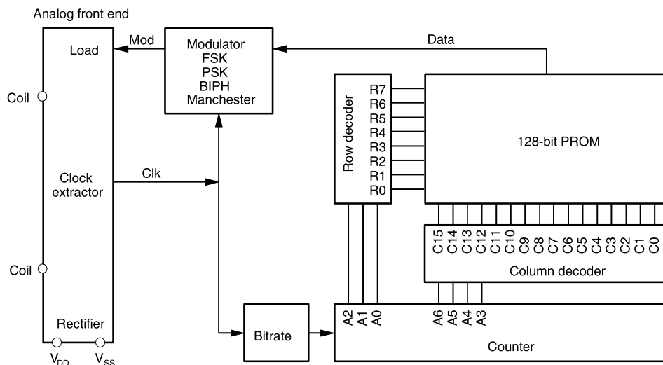
Figure 2. Block Diagram
