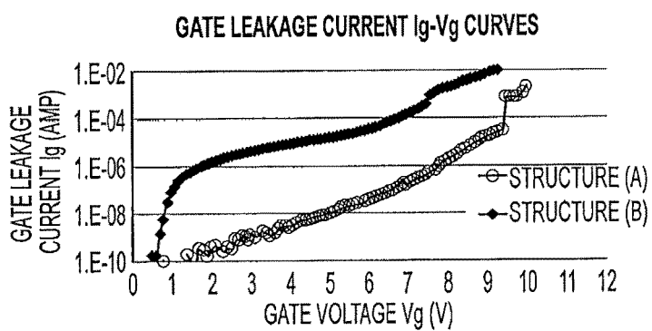
FIG. 4 PRIOR ART
