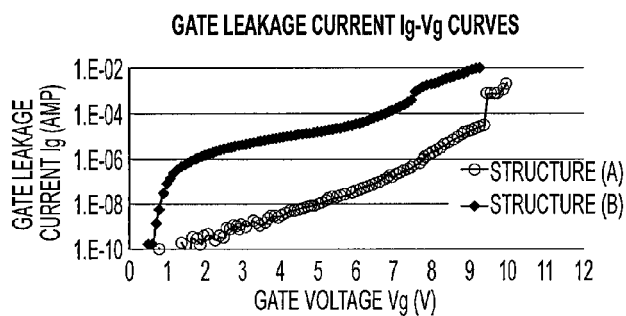
FIG. 4 PRIOR ART
