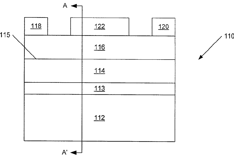
Figure 1 (PRIOR ART)
