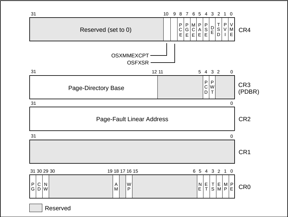
Figure 2-5. Control Registers
