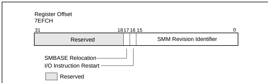
Figure 12-2. SMM Revision Identifier
