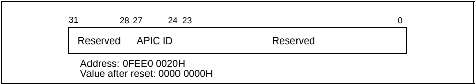
Figure 7-5. Local APIC ID Register
