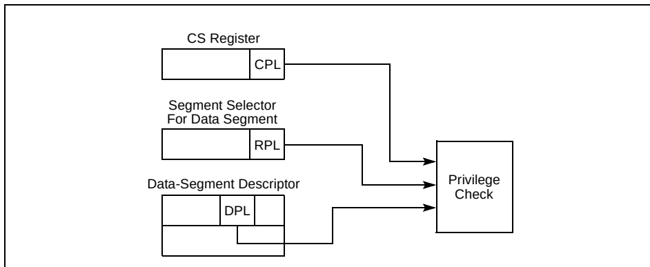
Figure 4-3. Privilege Check for Data Access
