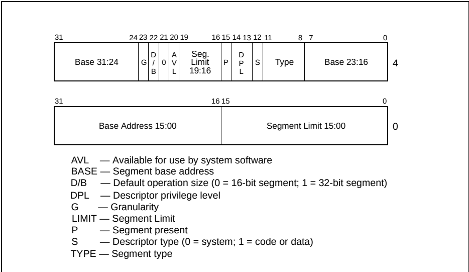
Figure 3-8. Segment Descriptor
