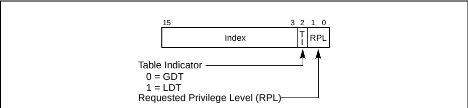
Figure 3-6. Segment Selector
