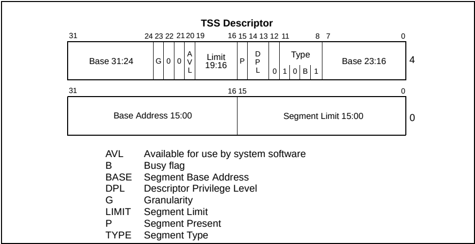
Figure 6-3. TSS Descriptor
