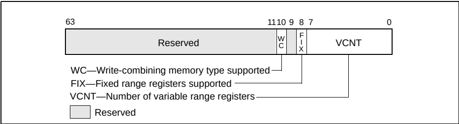
Figure 9-4. MTRRcap Register
