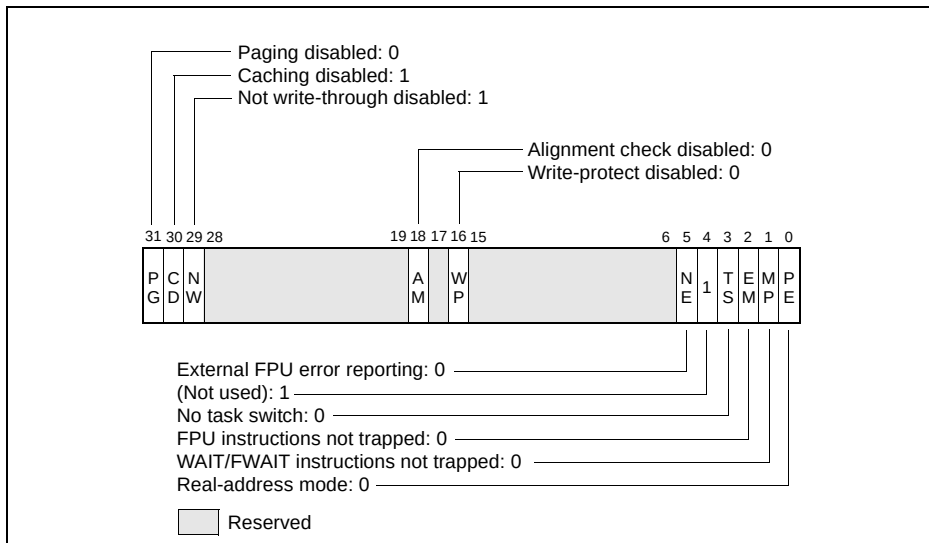
Figure 8-1. Contents of CR0 Register after Reset
