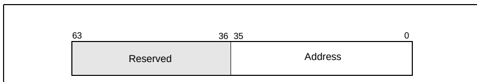
Figure 13-6. Machine-Check Bank Address Register
