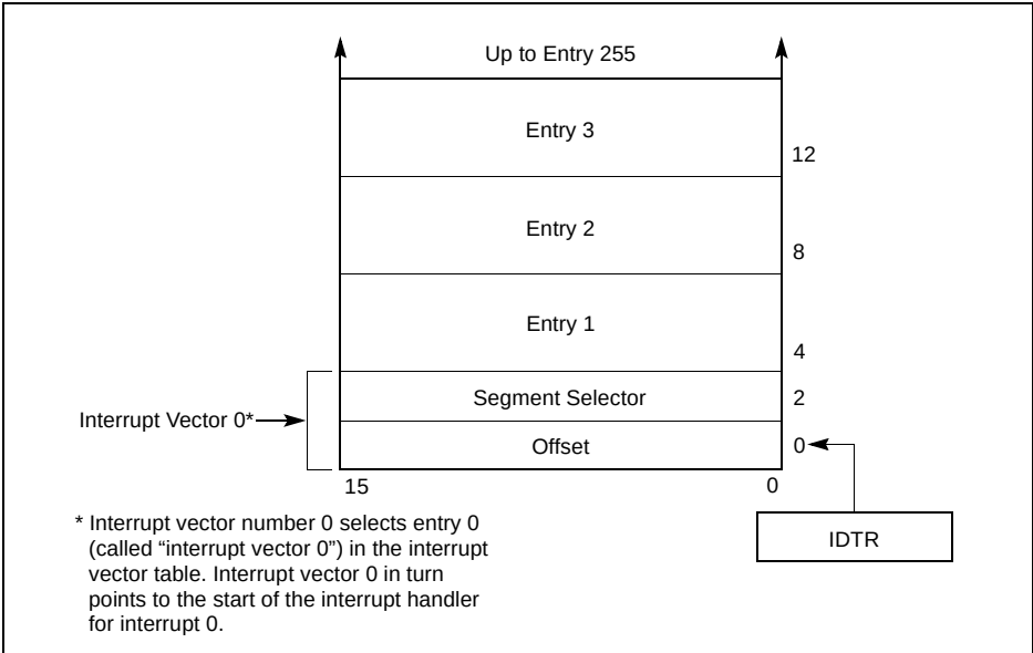
Figure 16-2. Interrupt Vector Table in Real-Address Mode
