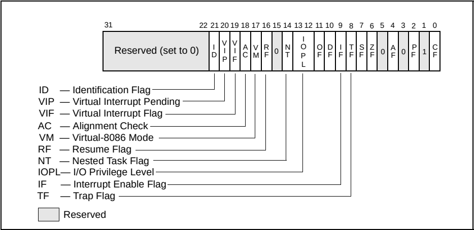
Figure 2-3. System Flags in the EFLAGS Register
