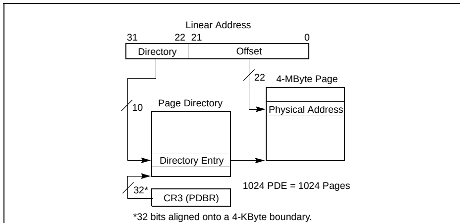
Figure 3-13. Linear Address Translation (4-MByte Pages)
