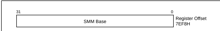
Figure 12-4. SMBASE Relocation Field
