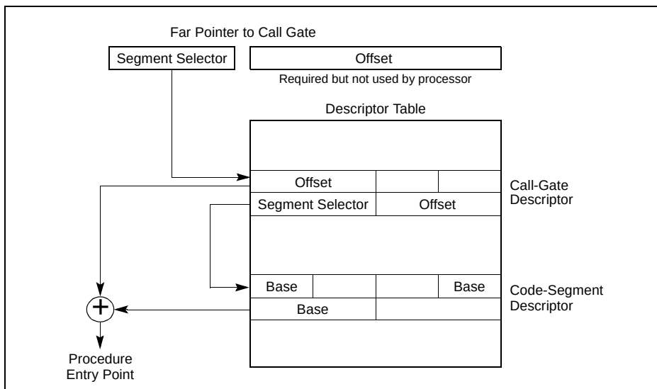
Figure 4-8. Call-Gate Mechanism
