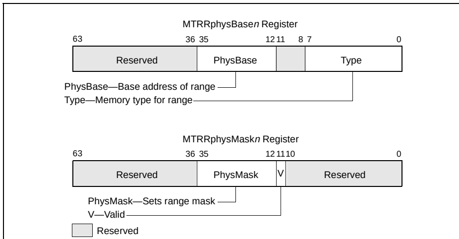
Figure 9-6. MTRRphysBasen and MTRRphysMaskn Variable-Range Register Pair
