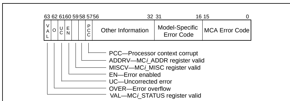
Figure 13-5. MCI_STATUS Register
