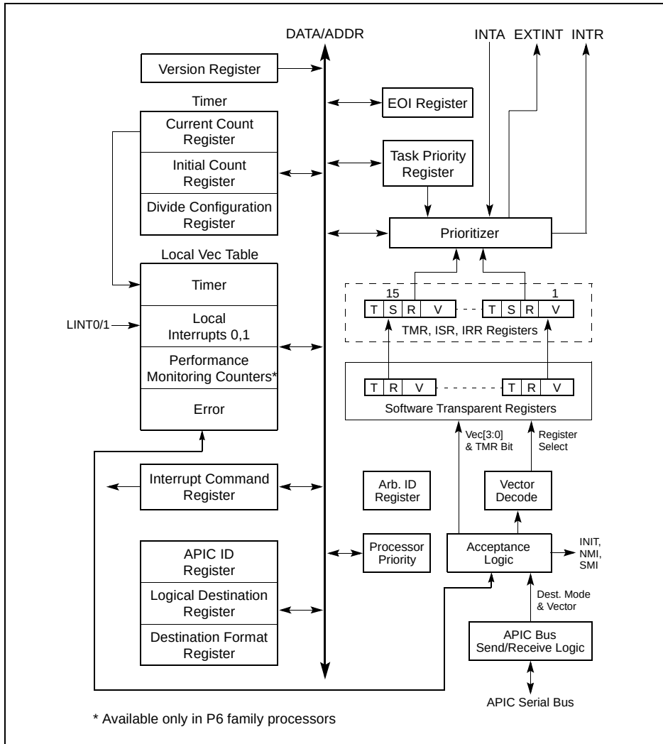
Figure 7-3. Local APIC Structure
