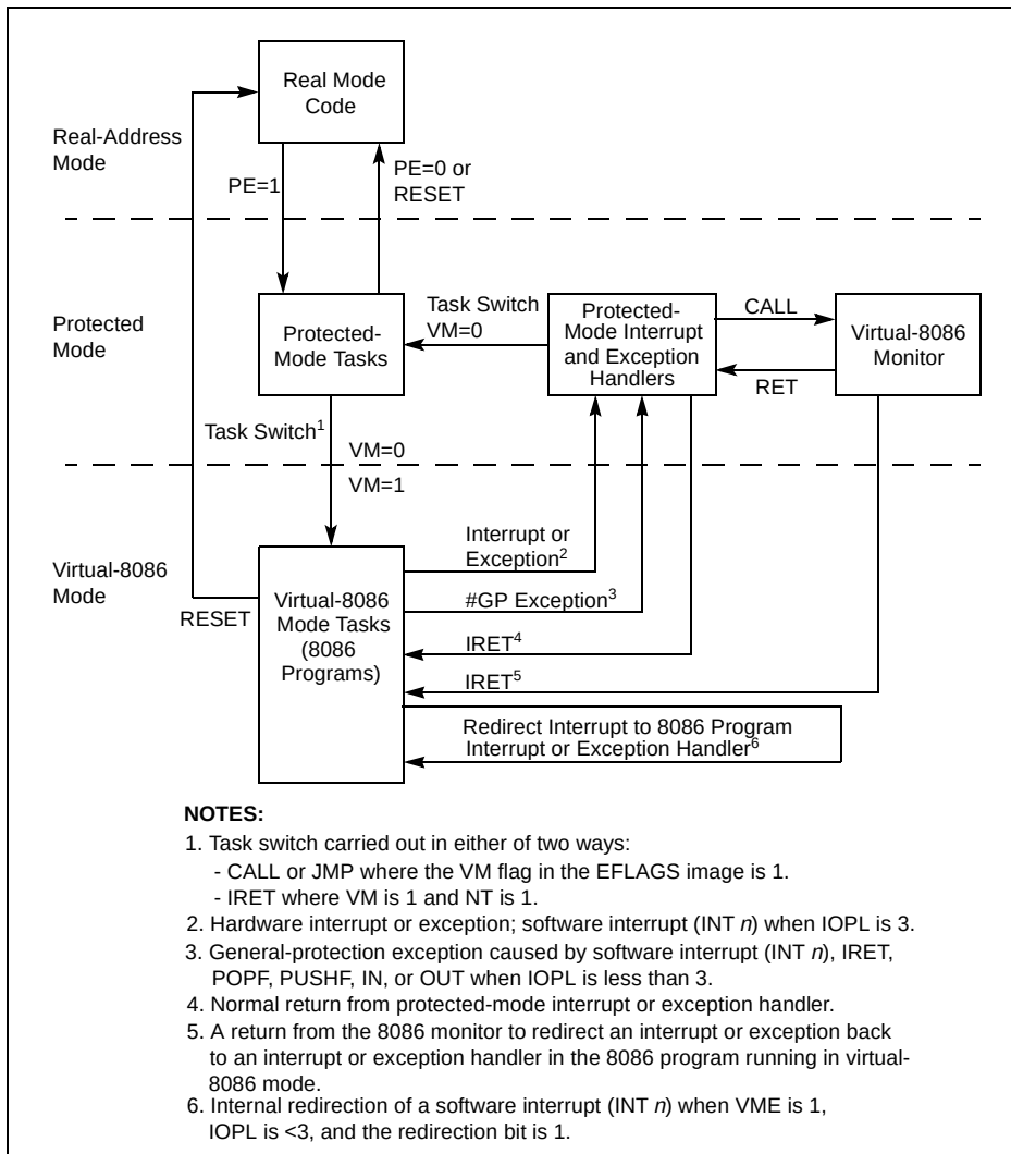
Figure 16-3. Entering and Leaving Virtual-8086 Mode
