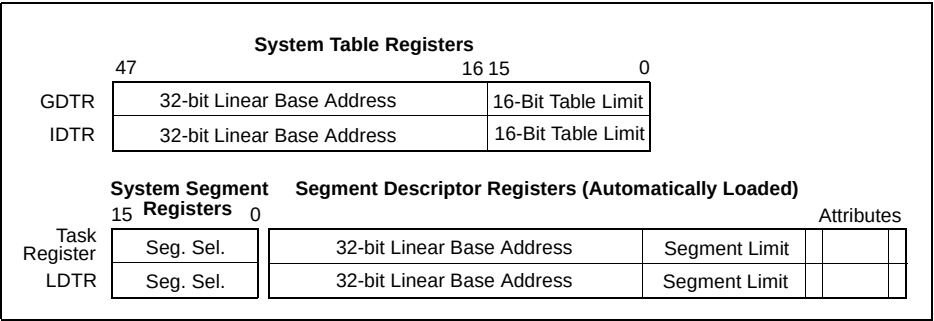
Figure 2-4. Memory Management Registers
