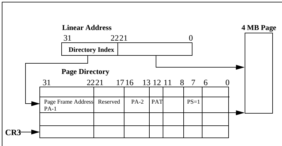
Figure 3-23. Page Size Extension Linear to Physical Translation
