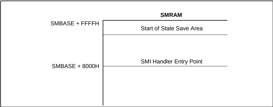
Figure 12-1. SMRAM Usage
