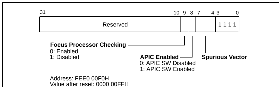
Figure 7-14. Spurious-Interrupt Vector Register (SVR)
