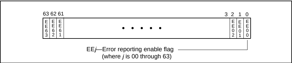
Figure 13-4. MCi_CTL Register
