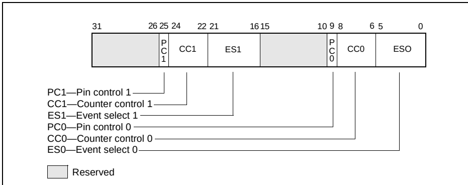
Figure 15-4. CESR MSR (Pentium® Processor Only)
