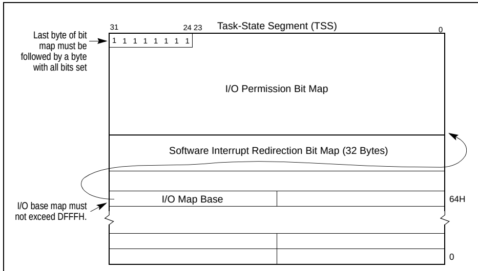
Figure 16-5. Software Interrupt Redirection Bit Map in TSS
