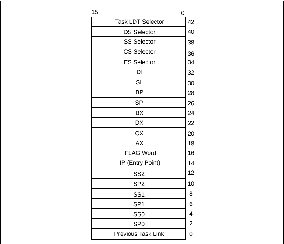
Figure 6-9. 16-Bit TSS Format
