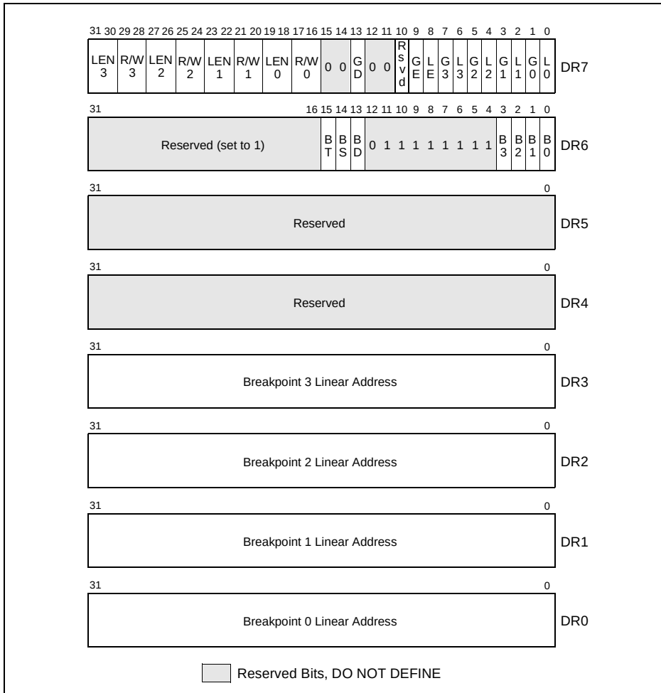
Figure 15-1. Debug Registers
