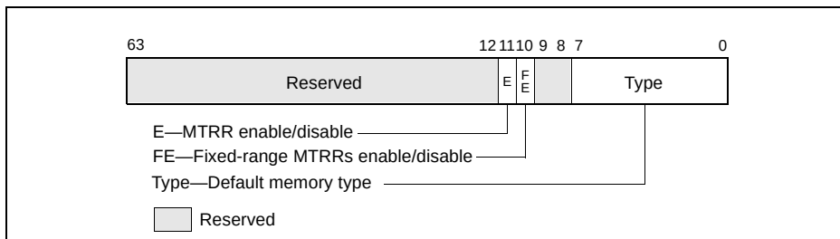
Figure 9-5. MTRRdefType Register
