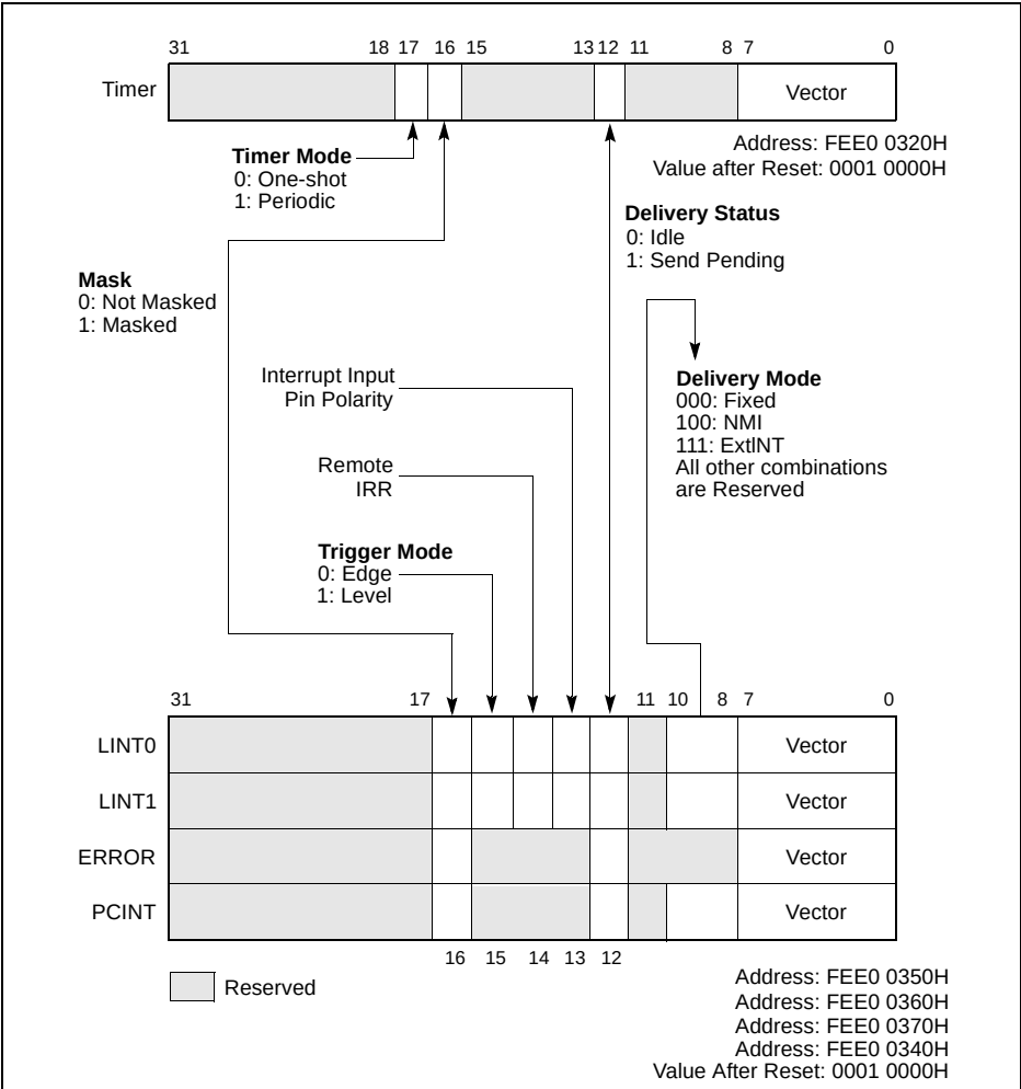
Figure 7-8. Local Vector Table (LVT)
