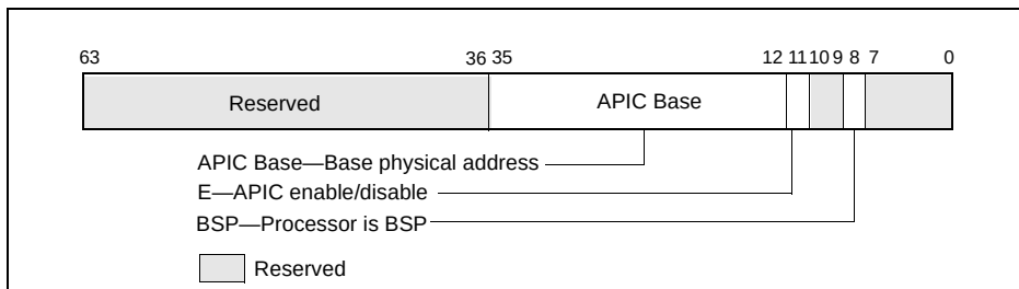
Figure 7-4. APIC_BASE_MSR
