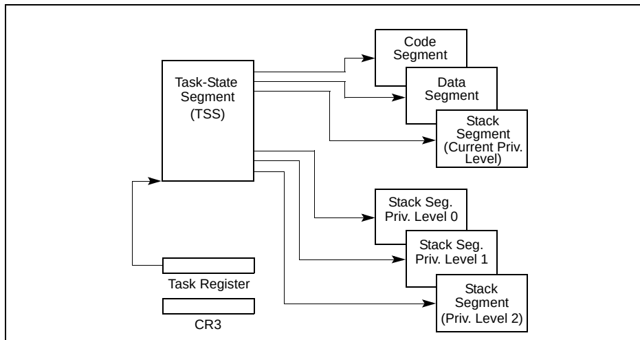
Figure 6-1. Structure of a Task
