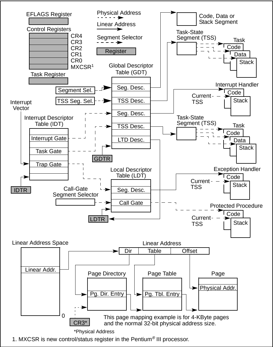
Figure 2-1. System-Level Registers and Data Structures
