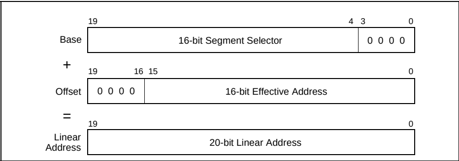
Figure 16-1. Real-Address Mode Address Translation
