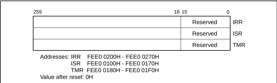
Figure 7-10. IRR, ISR and TMR Registers
