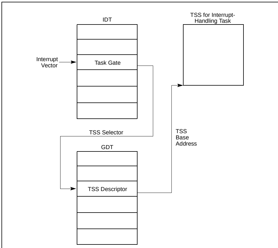
Figure 5-5. Interrupt Task Switch
