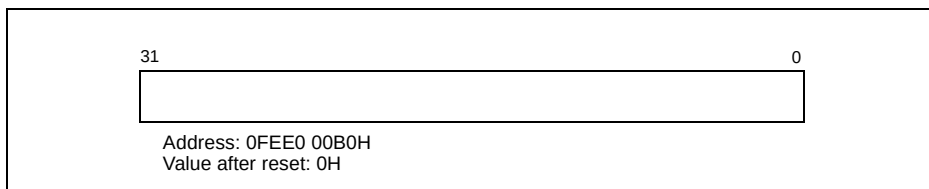
Figure 7-13. EOI Register
