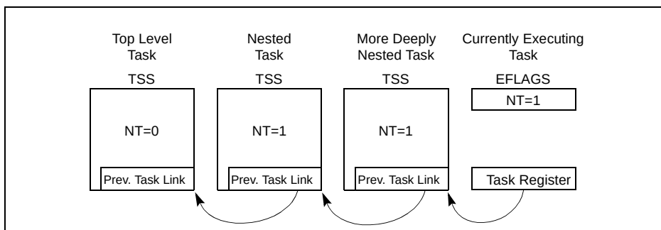
Figure 6-7. Nested Tasks
