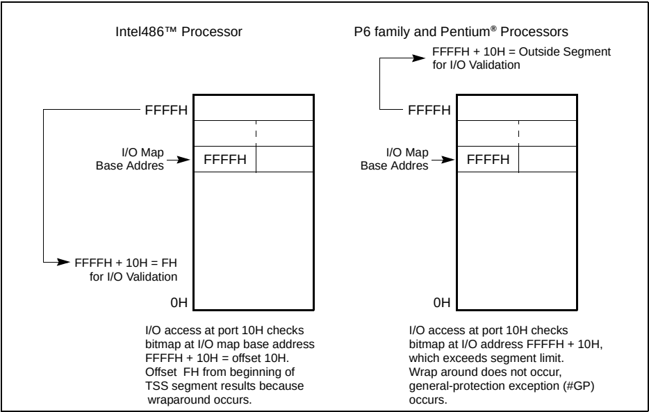
Figure 18-1. I/O Map Base Address Differences
