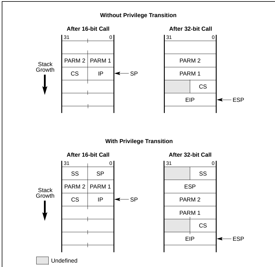
Figure 17-1. Stack after Far 16- and 32-Bit Calls
