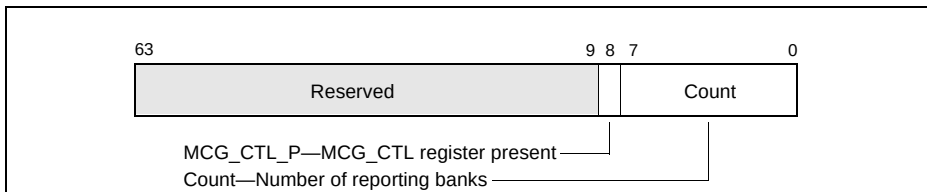
Figure 13-2. MCG_CAP Register
