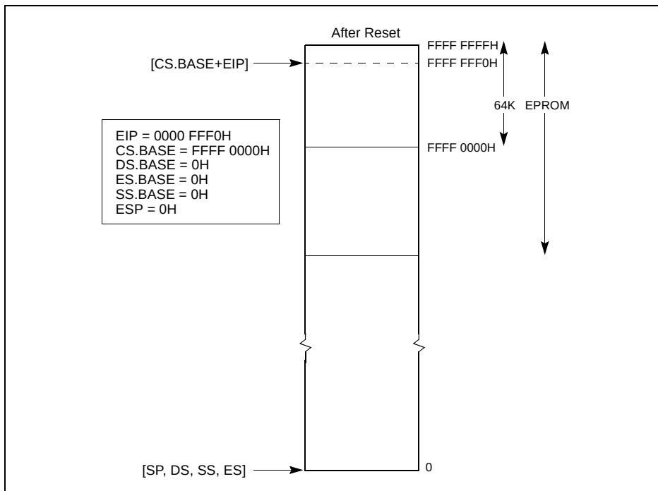
Figure 8-3. Processor State After Reset
