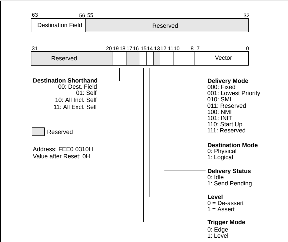
Figure 7-9. Interrupt Command Register (ICR)
