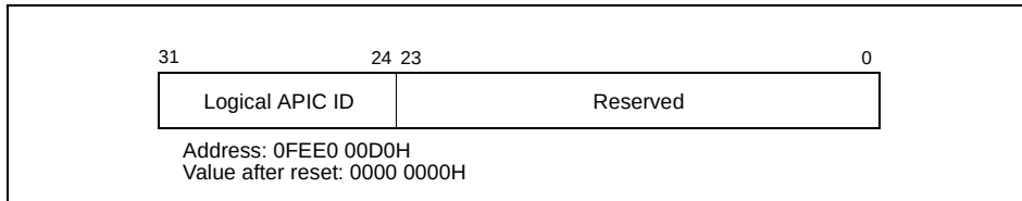
Figure 7-6. Logical Destination Register (LDR)
