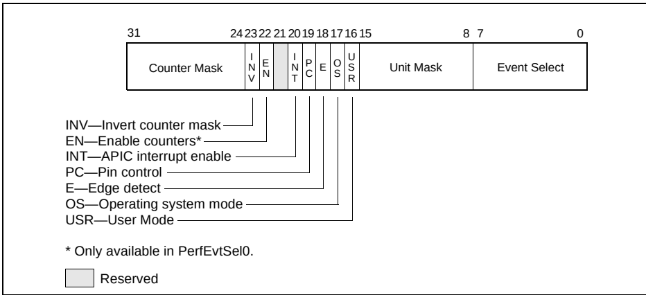
Figure 15-3. PerfEvtSel0 and PerfEvtSel1 MSRs
