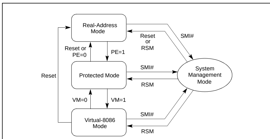
Figure 2-2. Transitions Among the Processor's Operating Modes
