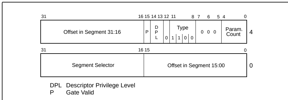
Figure 4-7. Call-Gate Descriptor
