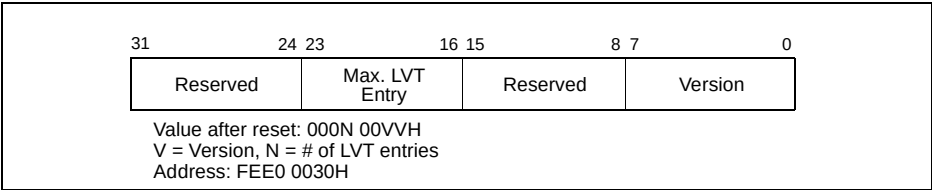
Figure 7-15. Local APIC Version Register
