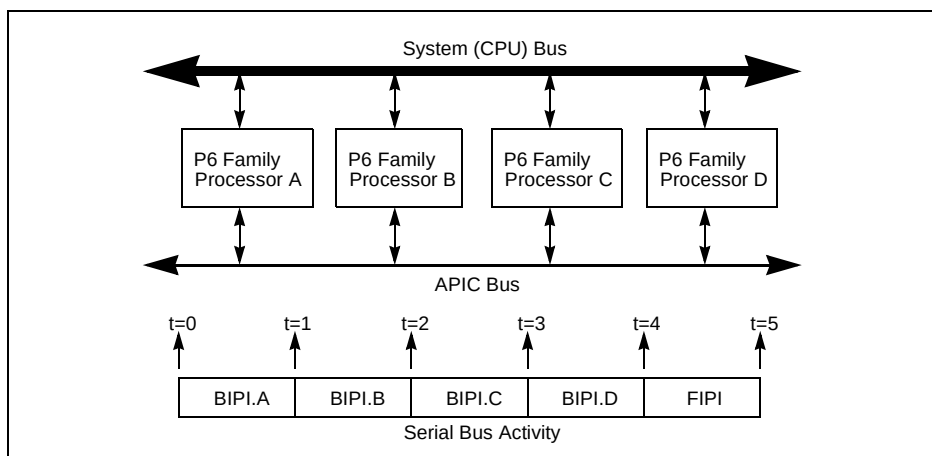
Figure 7-19. SMP System
