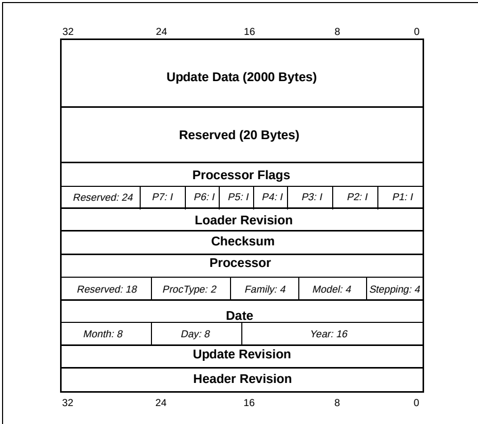
Figure 8-8. Format of the Microcode Update Data Block
