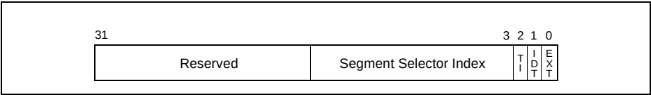
Figure 5-6. Error Code
