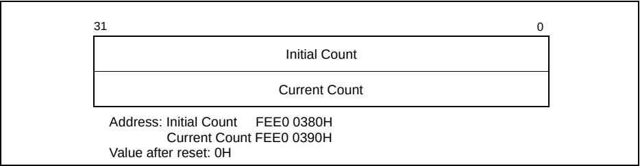
Figure 7-18. Initial Count and Current Count Registers
