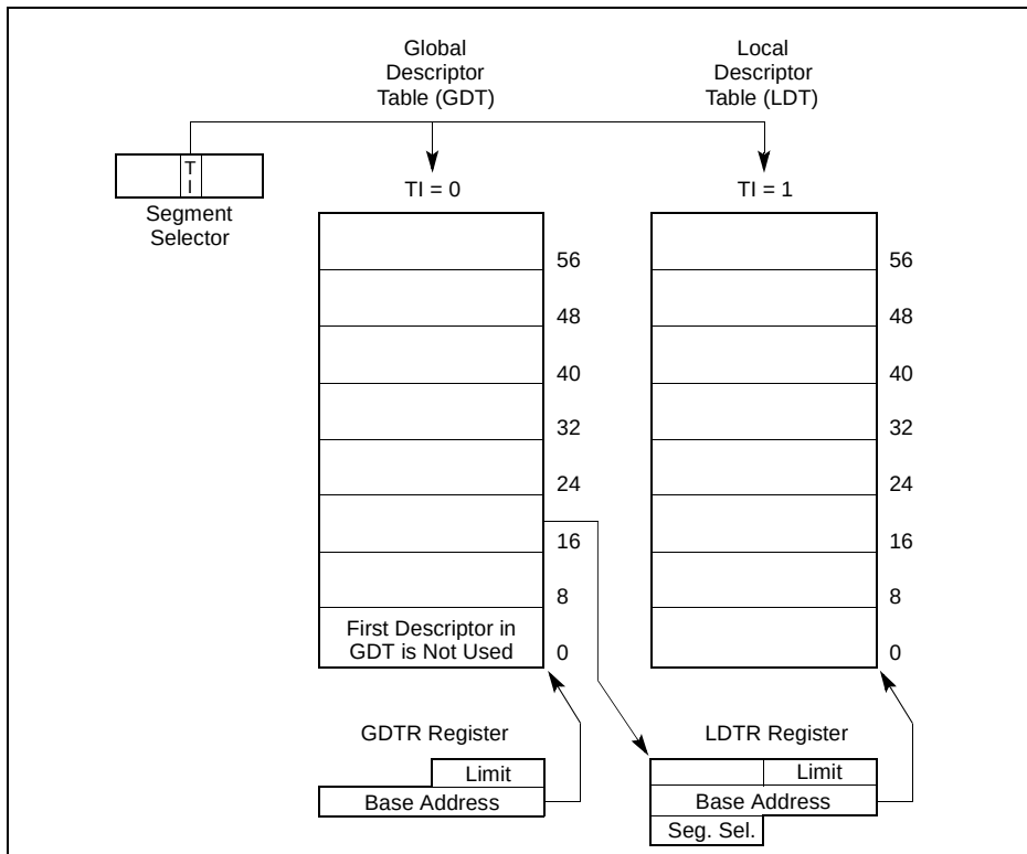
Figure 3-10. Global and Local Descriptor Tables
