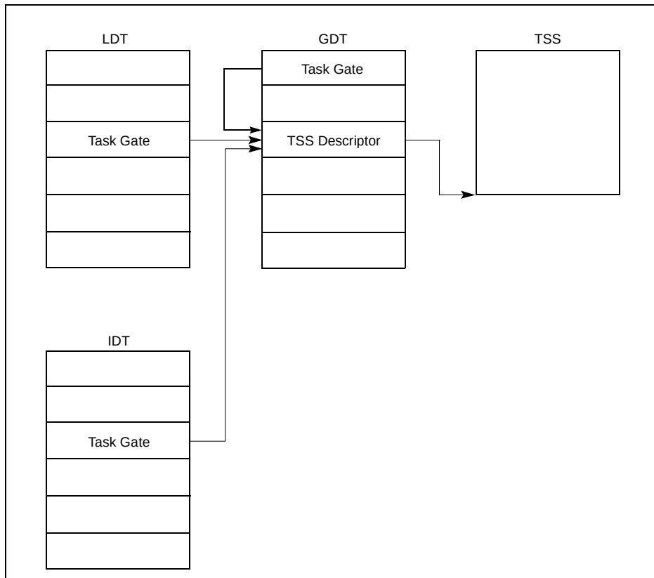
Figure 6-6. Task Gates Referencing the Same Task
