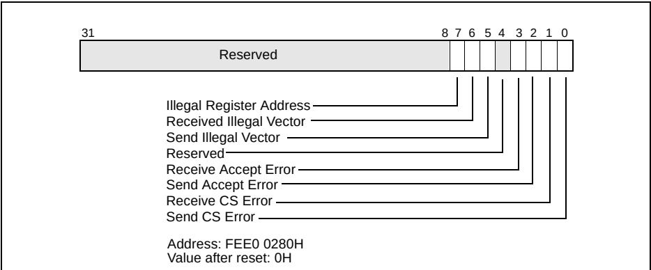
Figure 7-16. Error Status Register (ESR)
