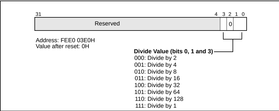
Figure 7-17. Divide Configuration Register
