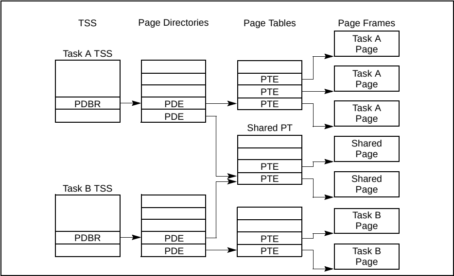
Figure 6-8. Overlapping Linear-to-Physical Mappings
