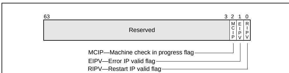
Figure 13-3. MCG_STATUS Register
