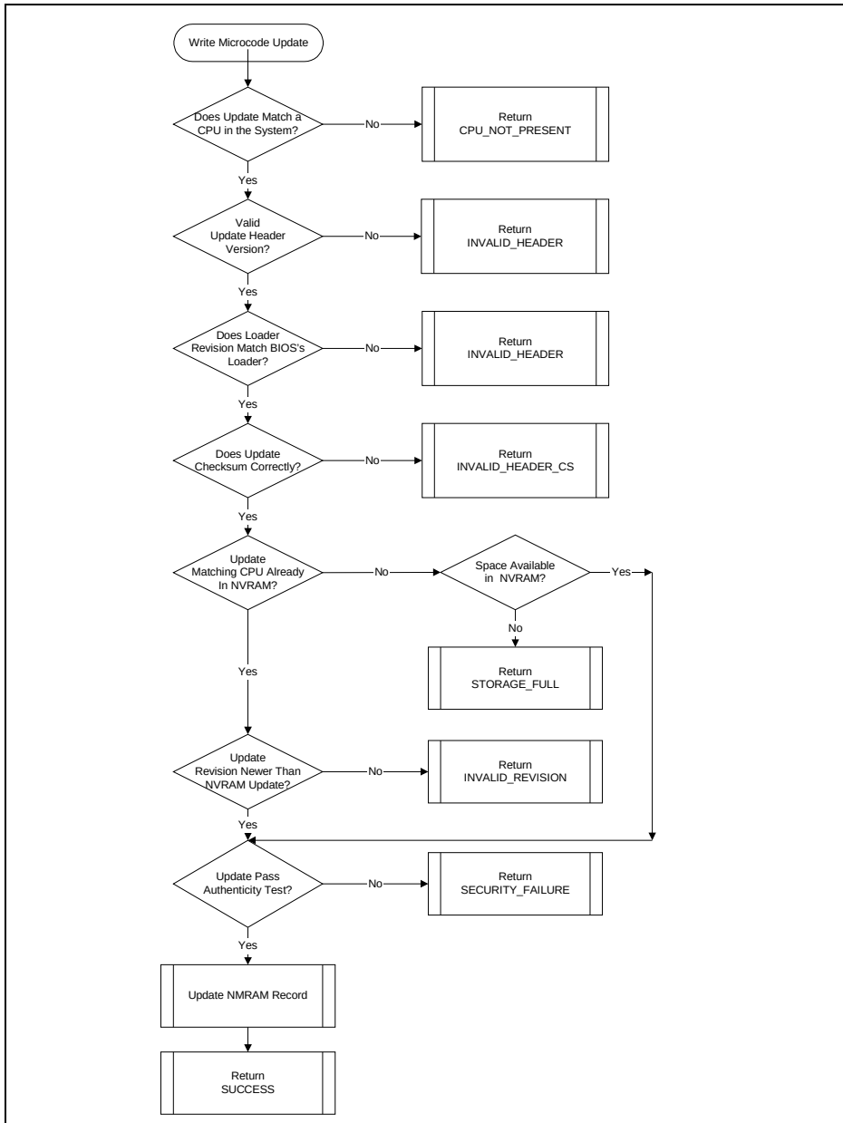
Figure 8-9. Write Operation Flow Chart
