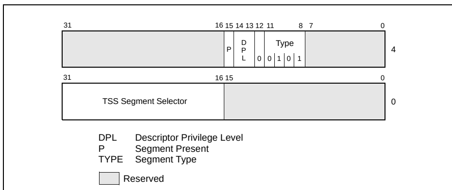
Figure 6-5. Task-Gate Descriptor
