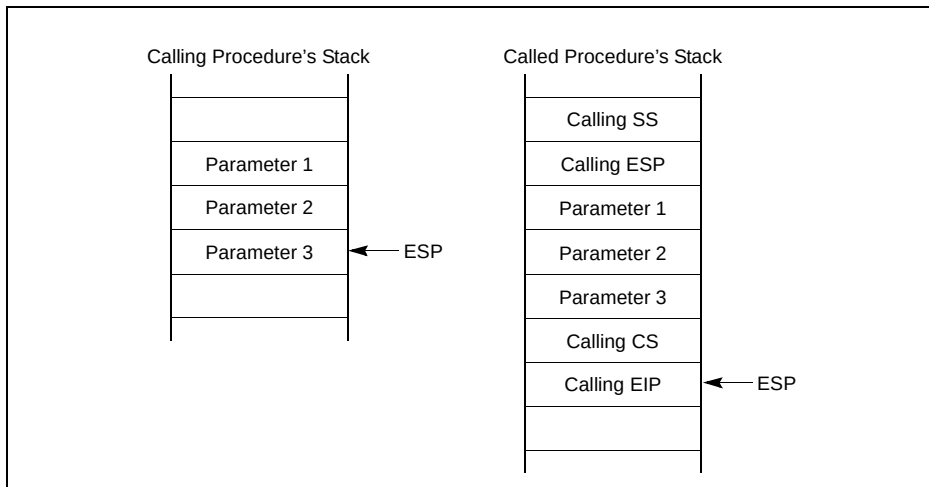
Figure 4-11. Stack Switching During an Interprivilege-Level Call
