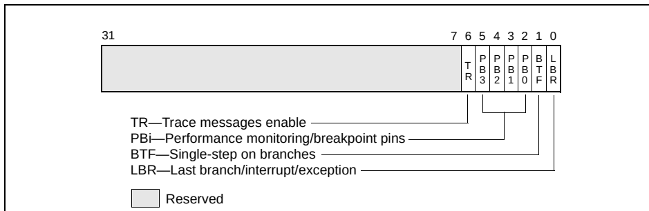
Figure 15-2. DebugCtlMSR Register
