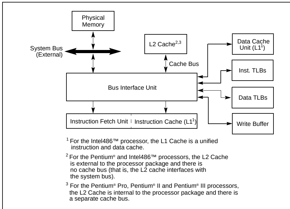
Figure 9-1. Intel Architecture Caches
