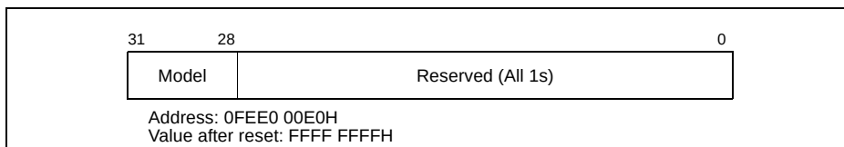
Figure 7-7. Destination Format Register (DFR)
