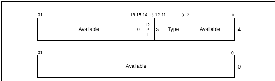
Figure 3-9. Segment Descriptor When Segment-Present Flag Is Clear
