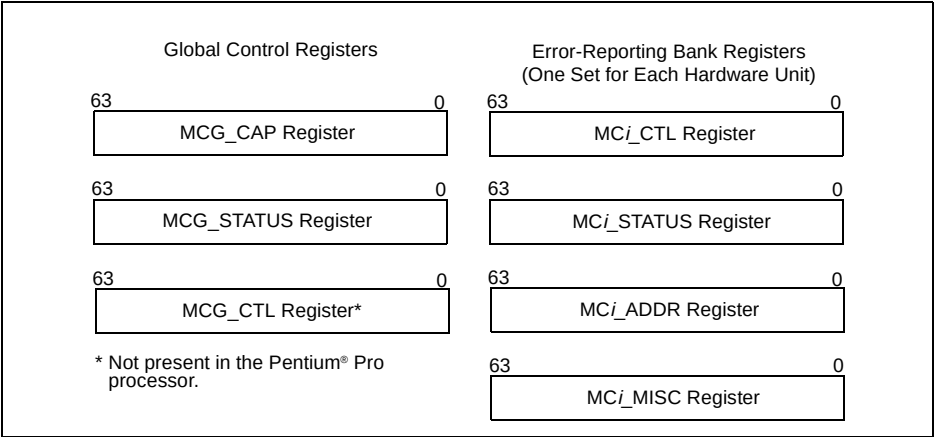
Figure 13-1. Machine-Check MSRs
