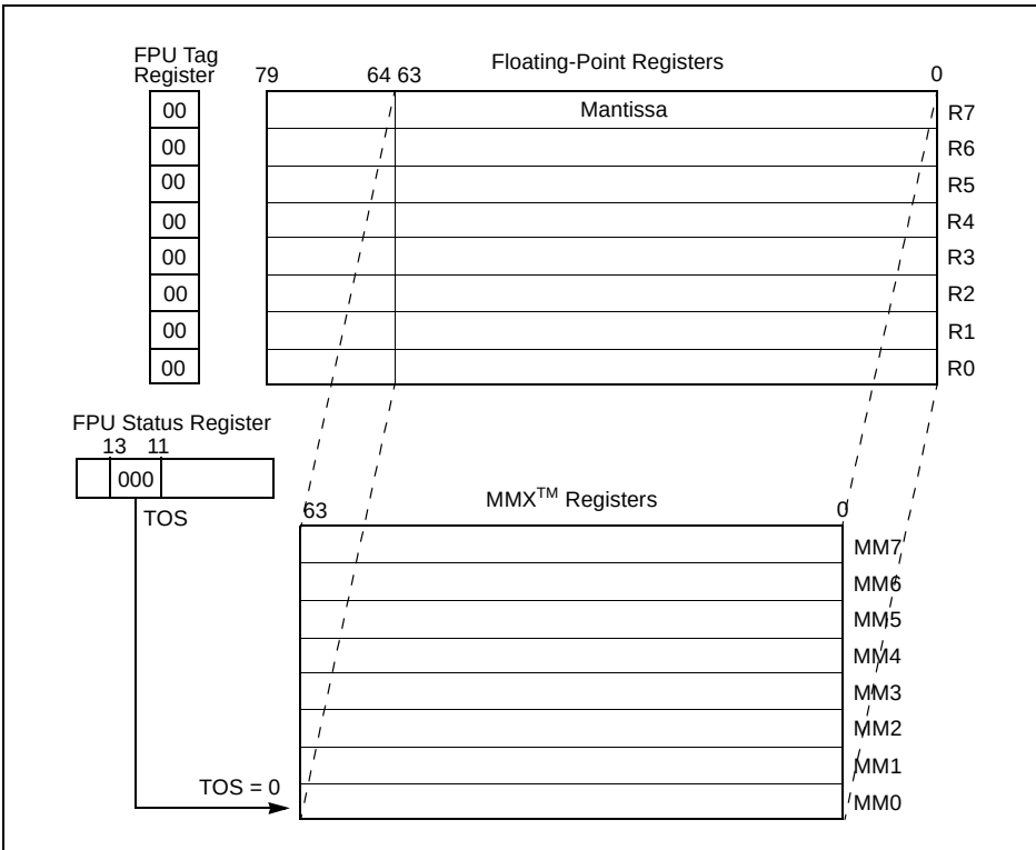
Figure 10-1. Mapping of MMX™ Registers to Floating-Point Registers
