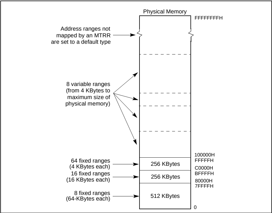
Figure 9-3. Mapping Physical Memory With MTRRs
