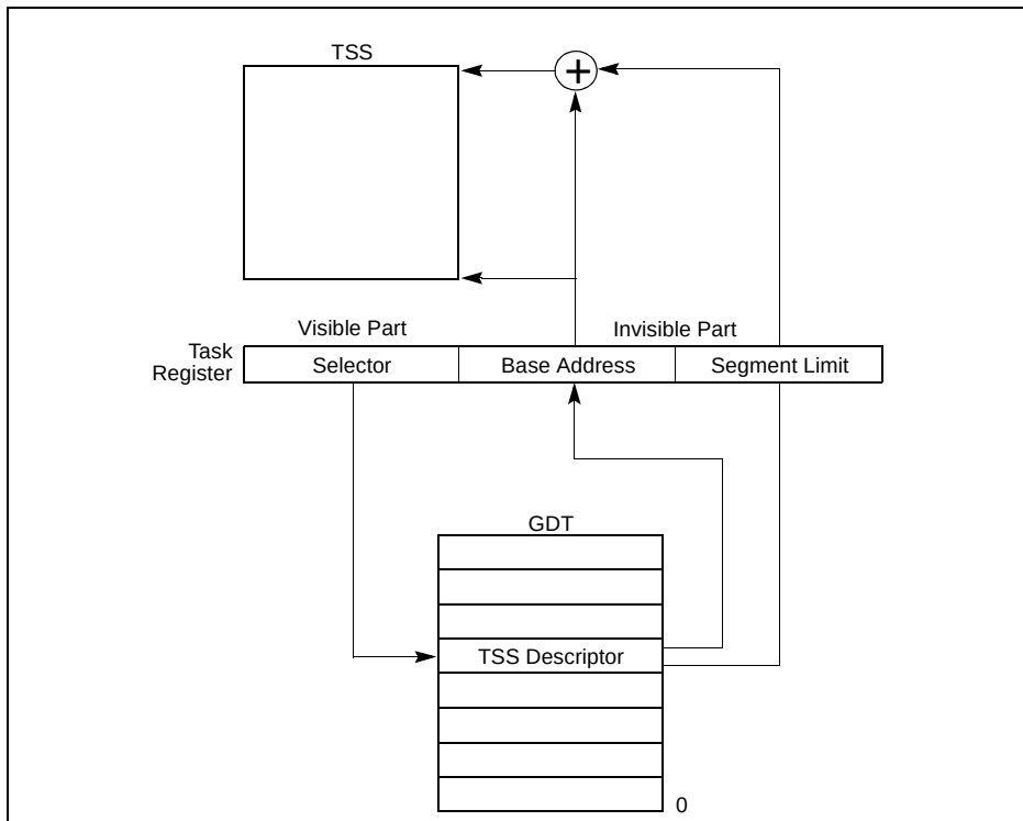
Figure 6-4. Task Register
