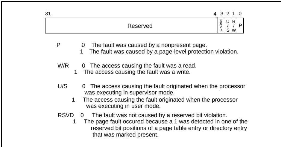
Figure 5-7. Page-Fault Error Code
