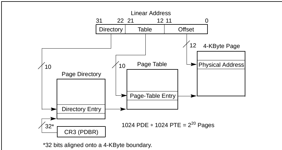
Figure 3-12. Linear Address Translation (4-KByte Pages)
