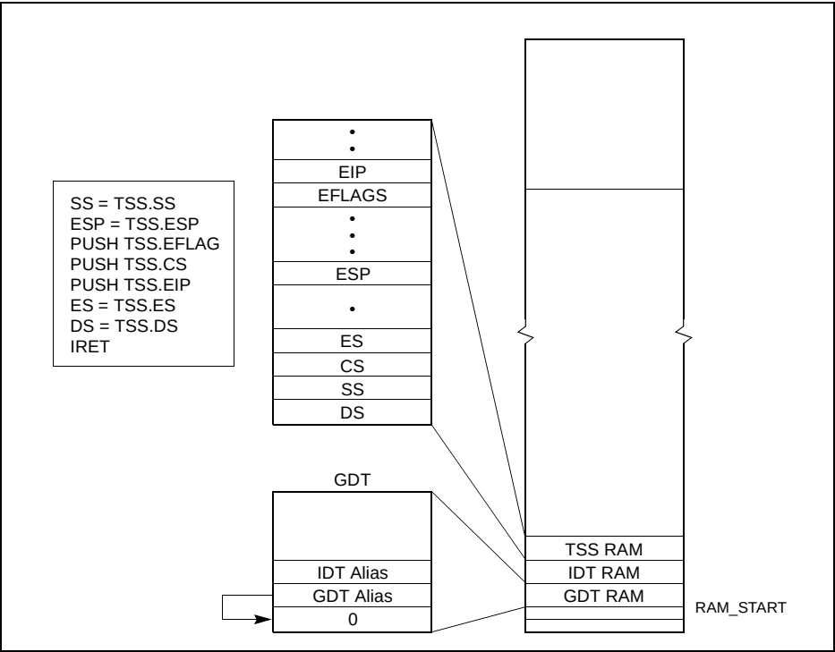
Figure 8-6. Task Switching (Lines 282-296 of List File)
