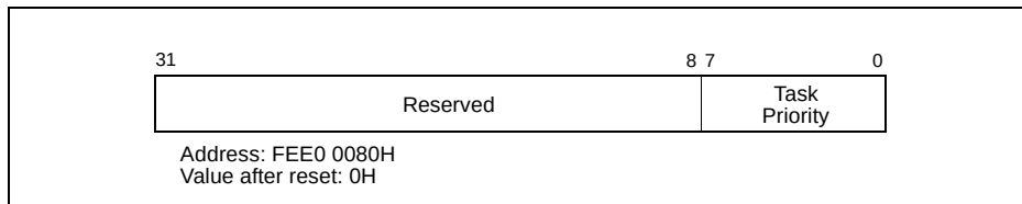
Figure 7-12. Task Priority Register (TPR)
