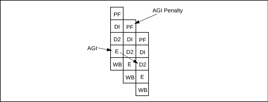
Figure 14-2. Pipeline Example of AGI Stall
