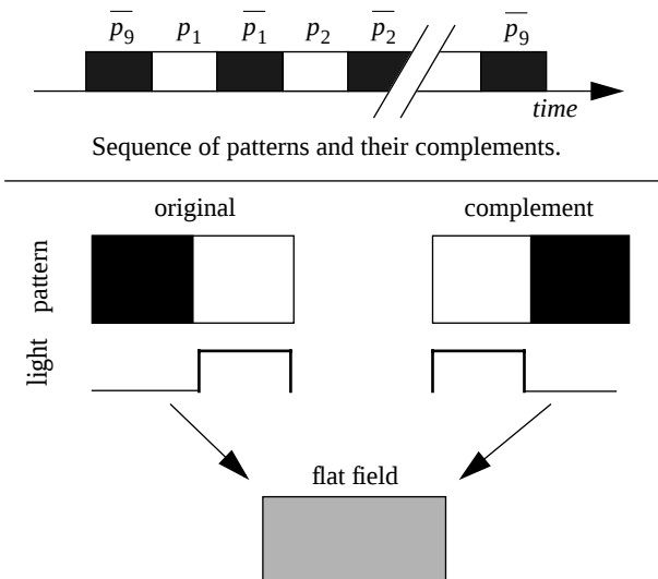
Figure 4: Pattern and complement are visually integrated over time, the result is the appearance of a flat field, or "white" light.
