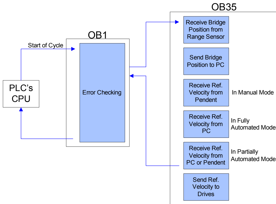
Figure 8: Cyclical architecture of the PLC control program.
