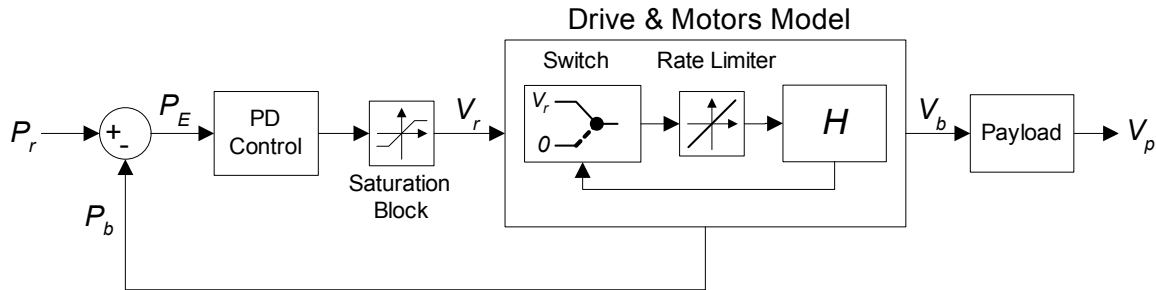
Figure 45: Block diagram of the positioning control module.
