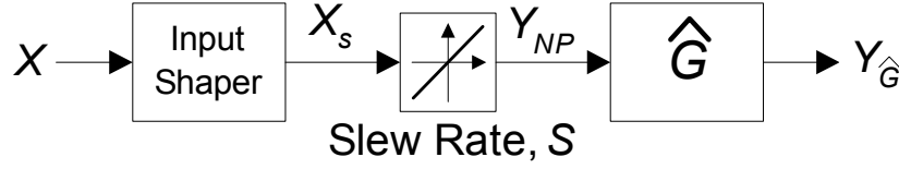
Figure 26: Generalized input shaping control with nonlinear rate limiter.
