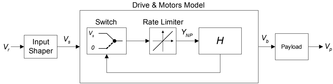
Figure 30: Input shaping control with drive and motors model.
