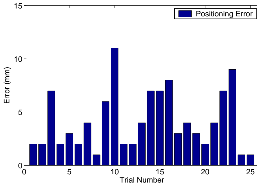
Figure 50: Positioning error for random moves throughout the crane workspace.
