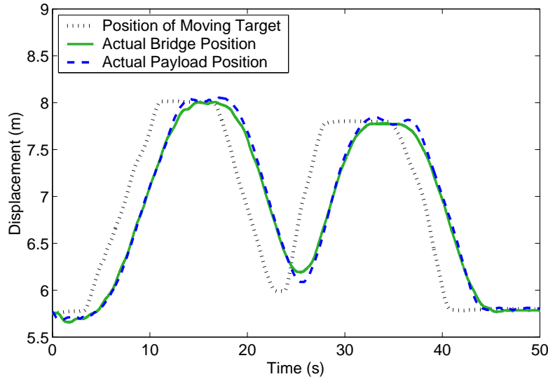
Figure 70: Response of the IPDC to a moving target position.
