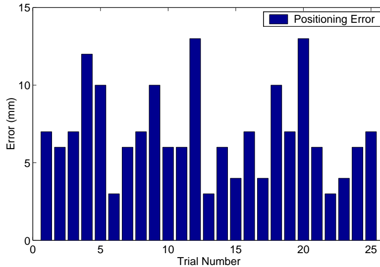
Figure 66: Final positioning error of the crane under the guidance of the input shaping and positioning controller.
