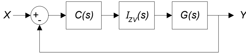
Figure 63: Simplified shaper-in-the-loop system.
