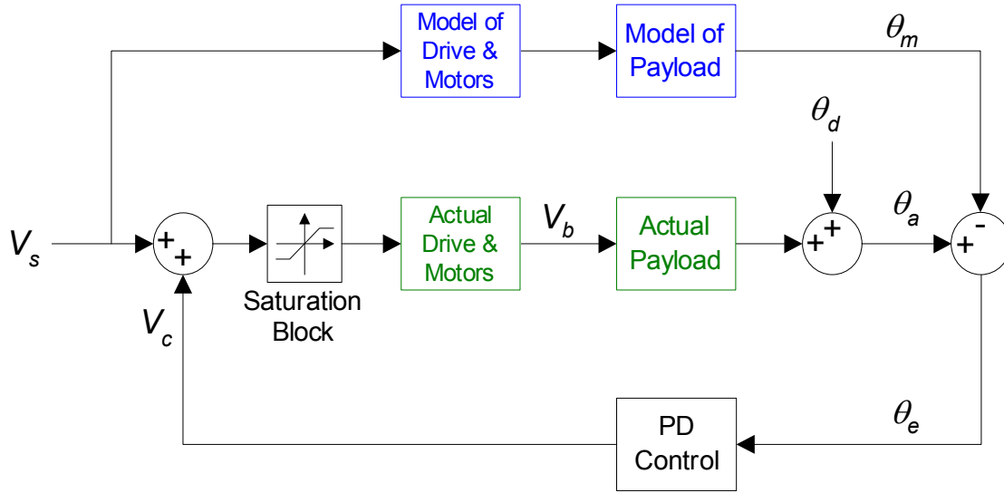
Figure 59: Model-augmented disturbance rejection control module.
