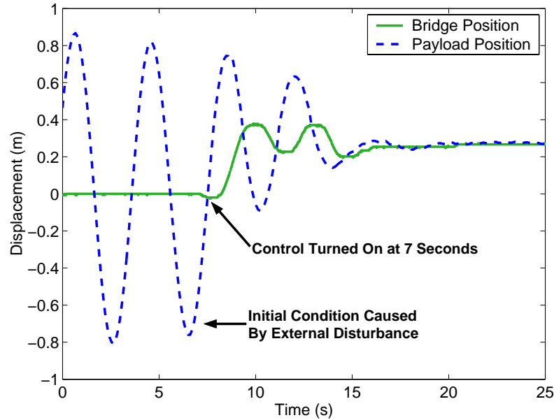
Figure 55: Cancellation of disturbance induced oscillations.
