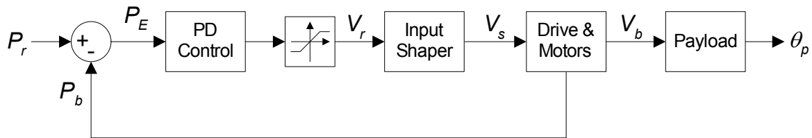
Figure 62: Combined input shaping and positioning controller.
