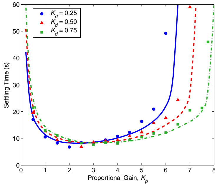
Figure 48: Experimental settling times for the positioning control module overlaid with the simulated settling times.
