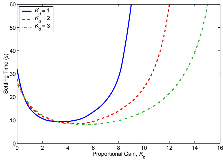
Figure 54: Simulated settling times for the disturbance rejection control module.
