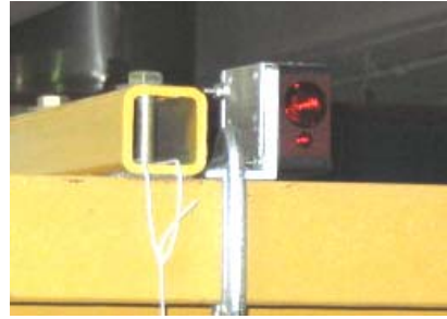
b) Laser range sensor.
