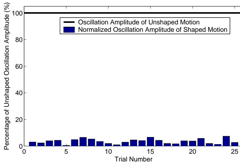
Figure 67: Residual payload oscillation amplitude of the crane under the guidance of the input shaping and positioning controller.
