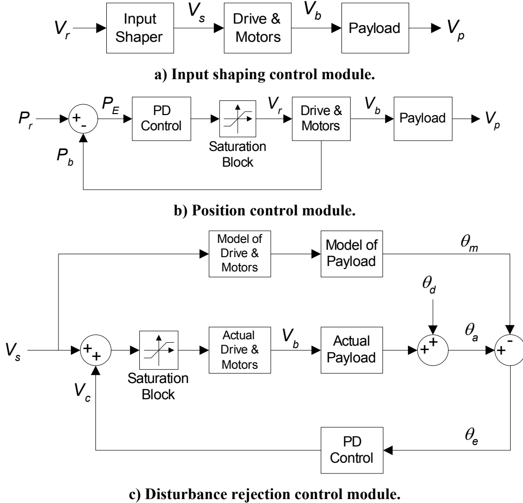
Figure 61: Individual control modules.
