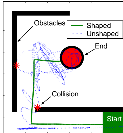
Figure 41: Obstacle course showing shaped and unshaped hook motions.
