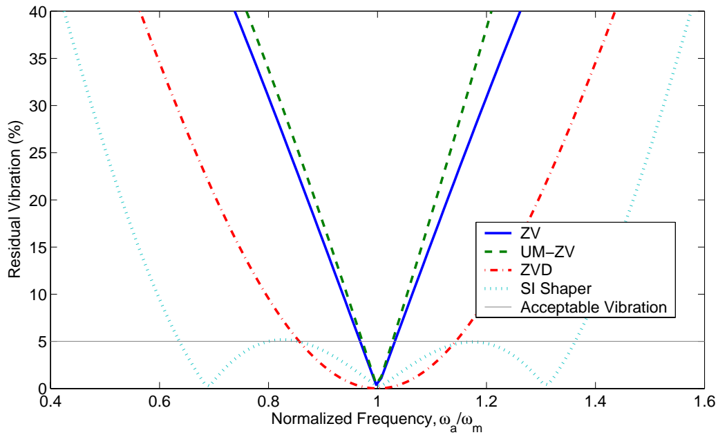
Figure 44: Robustness curves for some standard input shapers.
