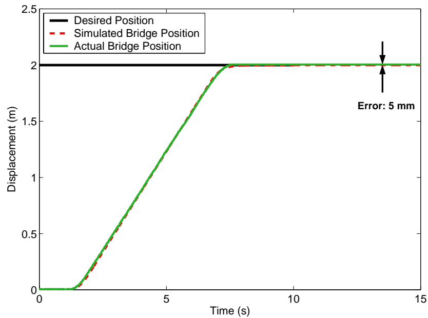
Figure 49: Actual and simulated bridge response to a reference command of 2 meters.
