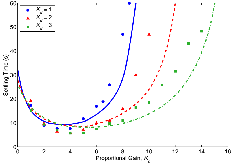
Figure 56: Experimental settling times for the disturbance rejection control module overlaid with the simulated settling times.
