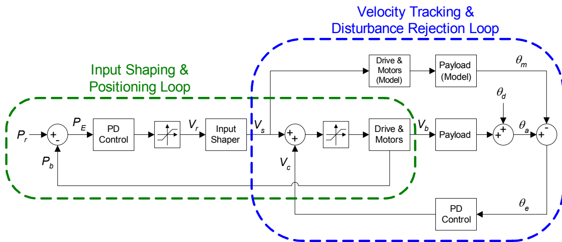
Figure 68: Combined input shaping, positioning, and disturbance rejection controller.
