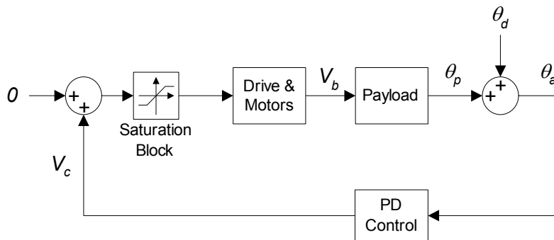
Figure 53: Disturbance rejection control module.
