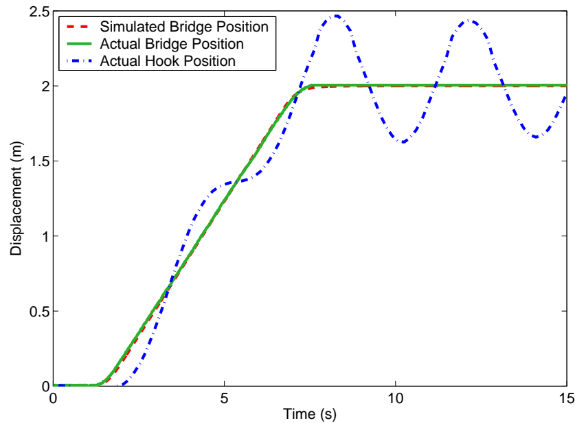
Figure 51: Actual and simulated bridge response to a reference command of 2 meters with the position of the hook shown.
