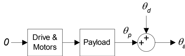
Figure 52: External disturbance affecting the output angle of the payload.
