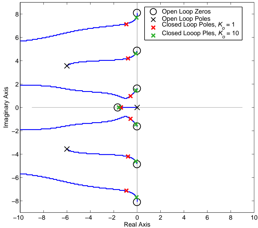
Figure 64: Root locus plot of linearized system.
