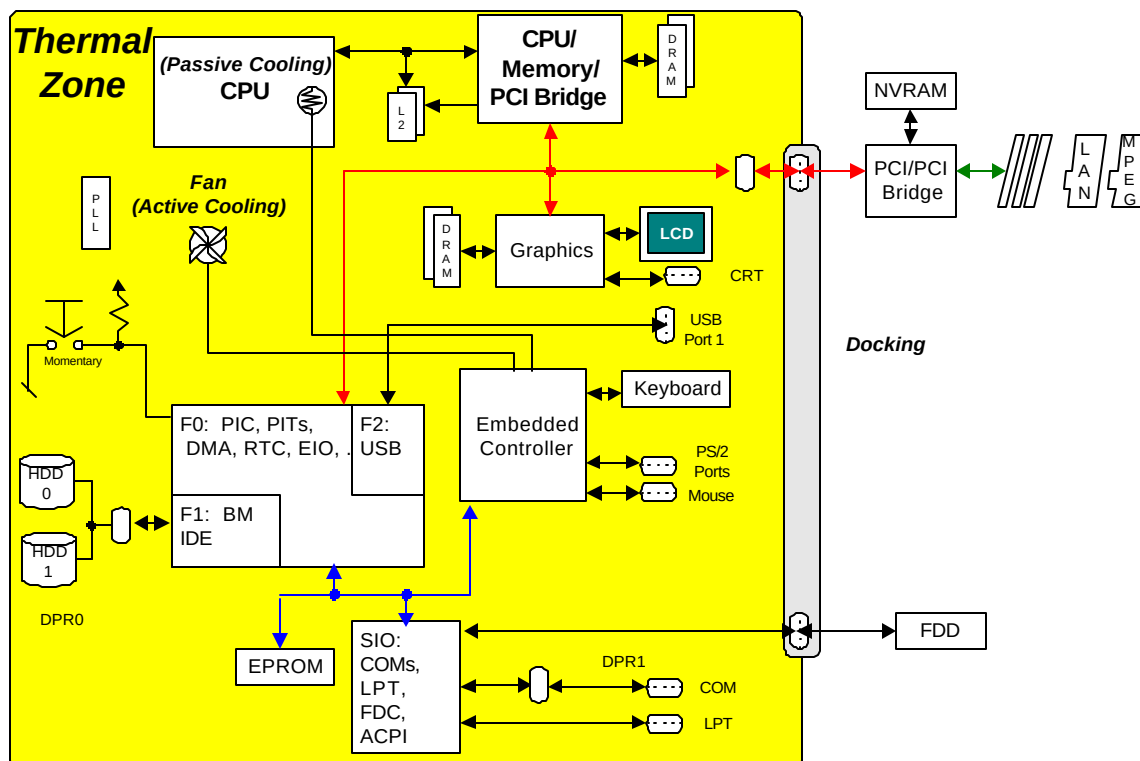
Figure 3-5 Thermal Zone
