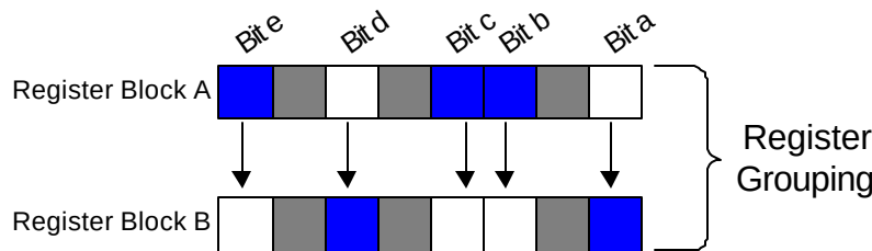
Figure 4-5 Example Fixed Hardware Feature Register Grouping
