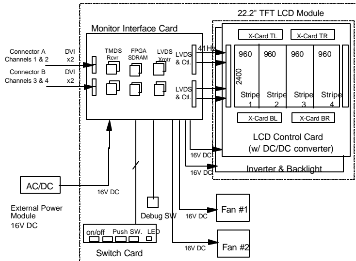
Figure 3. Block diagram of drive electronics.
