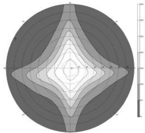
Figure 2 Polar plot of contrast ratio for dual-domain IPS, with 50:1 isocontours.
