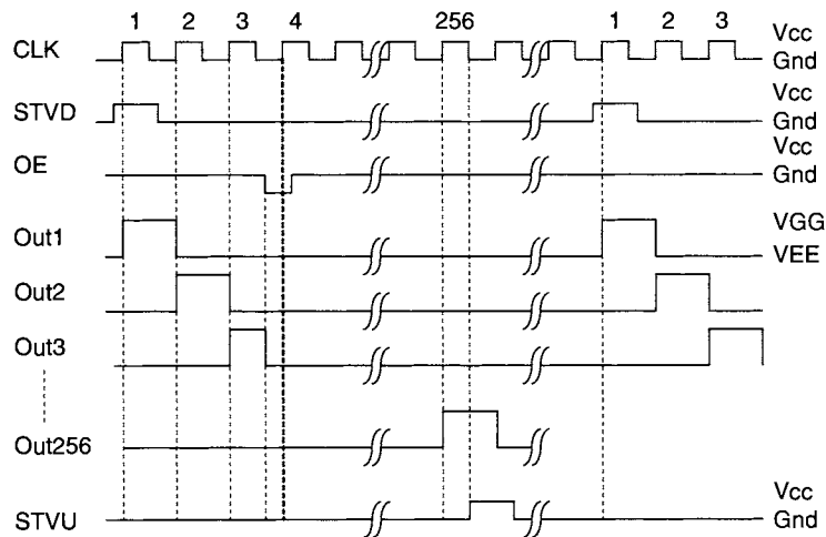
Figure 4.10: Timing diagram of a row driver.
