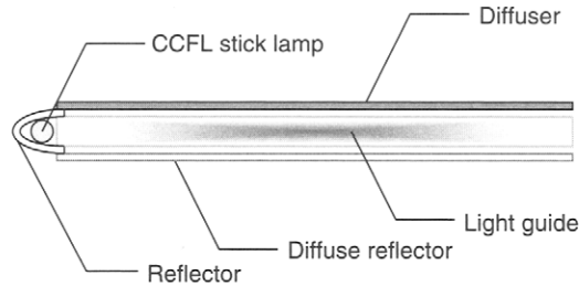
Figure 4.17: CCFL backlight configuration for notebook LCDs.
