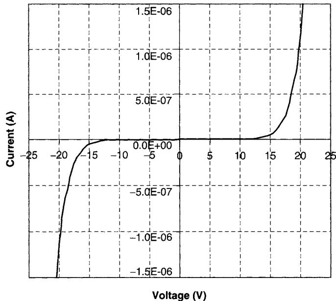
Figure 2.21: Linear current-voltage characteristic of \text{SiN}_x diode.
