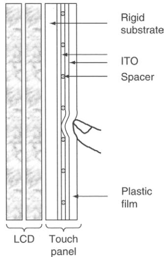
Figure 7.12: Resistive touch panel configuration.
