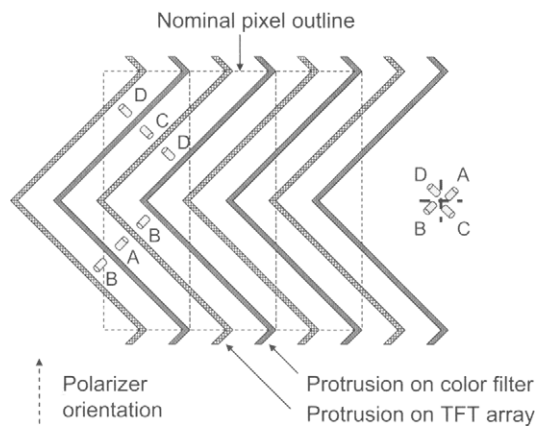
Figure 6.21: Protrusion design for a four-domain MVA LCD [8].
