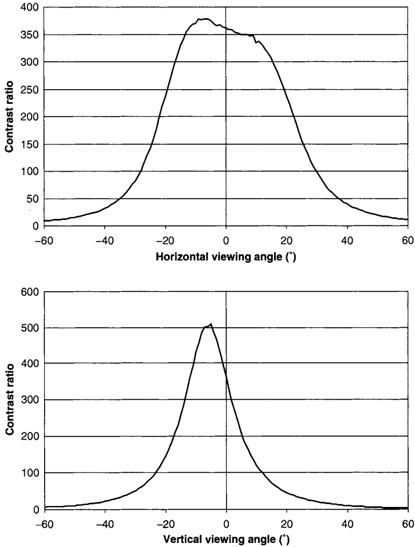
Figure 5.6: Dependence of contrast ratio on viewing angle in a typical TN AMLCD.
