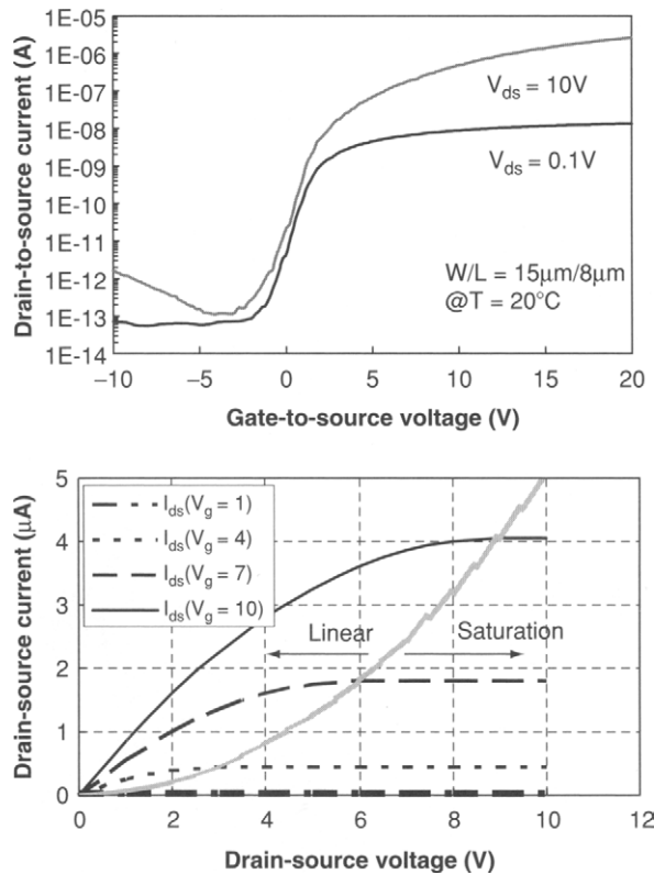
Figure 2.9: Current-voltage characteristics of a-Si TFT.
