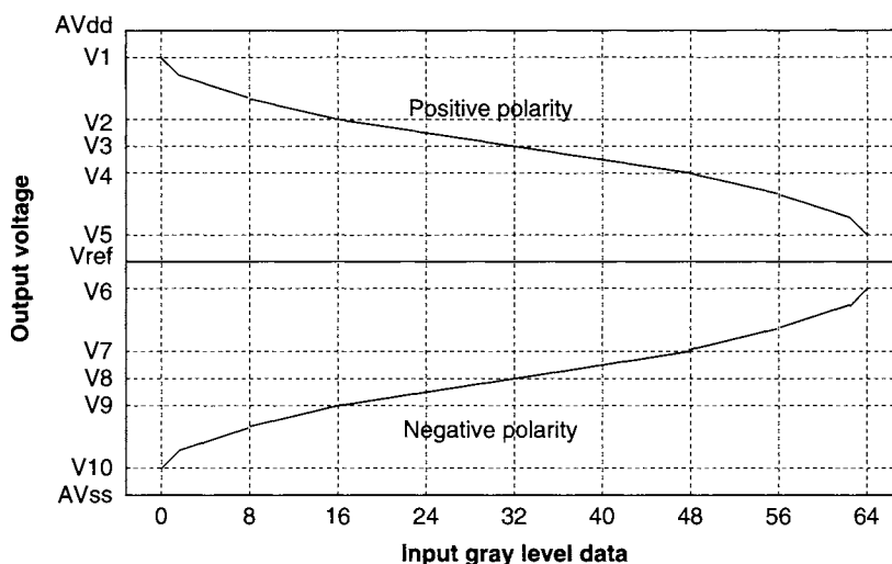
Figure 4.7: Gamma correction diagram.
