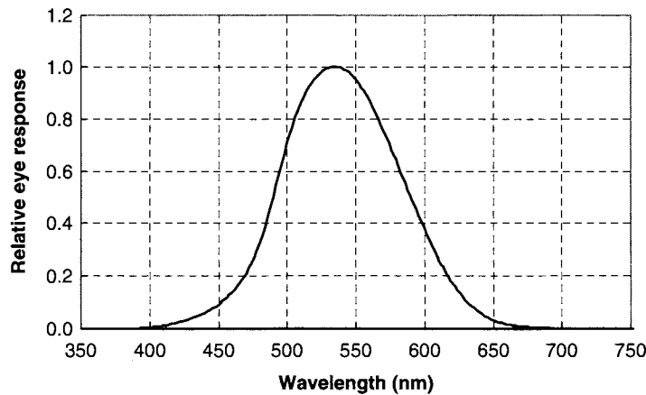
Figure 5.1: Eye response or photopic luminous efficiency curve.
