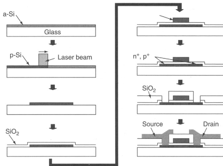
Figure 3.17: Basic sequence of a poly-Si TFT process.
