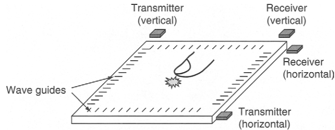
Figure 7.16: Operating principle of a SAW touch screen.
