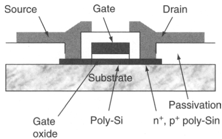
Figure 2.13: Cross section of poly-Si TFT.
