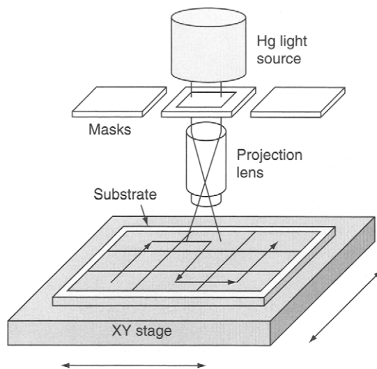
Figure 3.8: Flat panel stepper operating principle.
