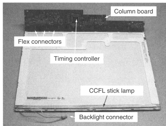
Figure 4.13: View of back of a TFT LCD module for notebook displays.
