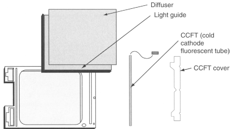
Figure 3.27: Final module assembly.
