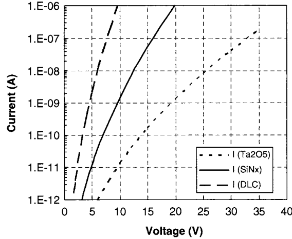
Figure 2.22: Typical semi-logarithmic current-voltage characteristics of Ta2O5, Si-rich SiNx and diamond-like carbon (DLC) diodes (reprinted with permission from the Society for Information Display).
