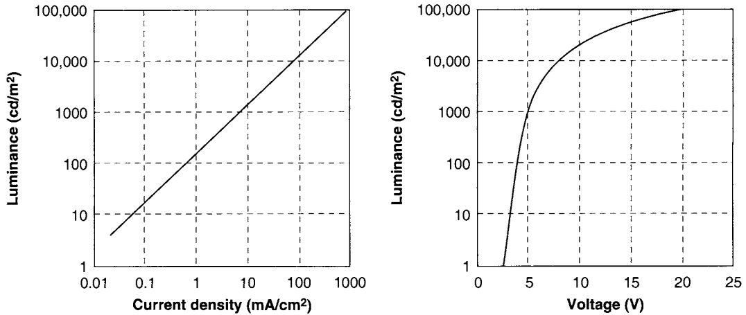
Figure 8.7: Luminance characteristics of Alq3-based OLED.
