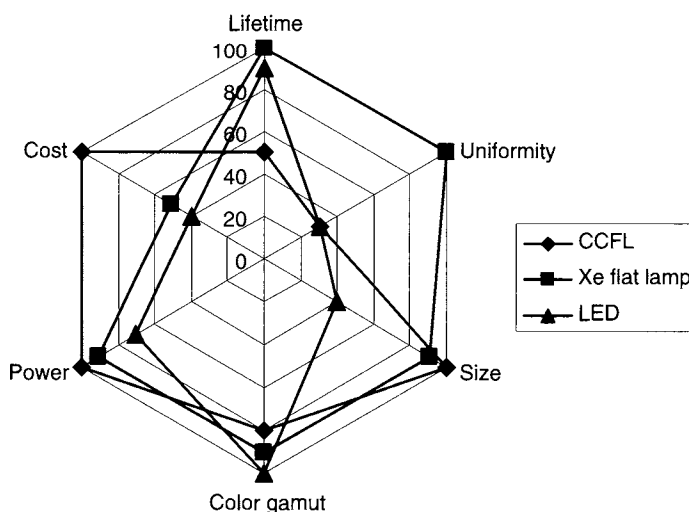
Figure 4.19: Comparison of different backlight technologies.
