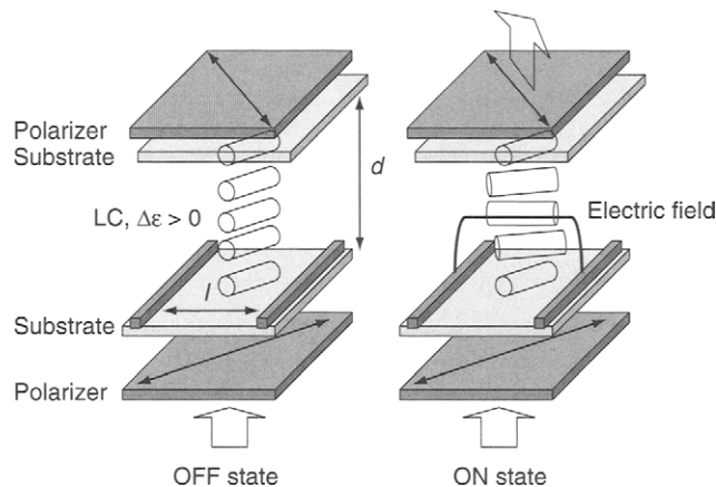
Figure 6.14: Operating principle of in-plane switching.
