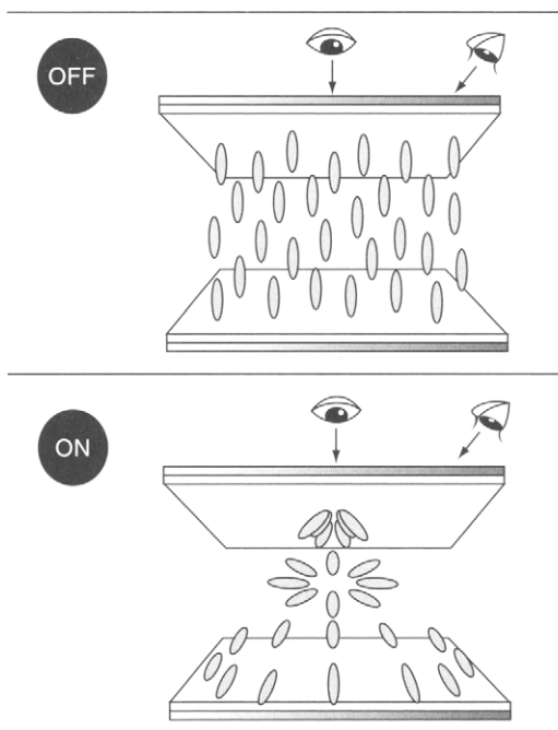
Figure 6.25: Operating principle of the ASV mode.
