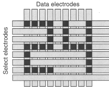
Figure 1.13: Passive matrix addressing.
