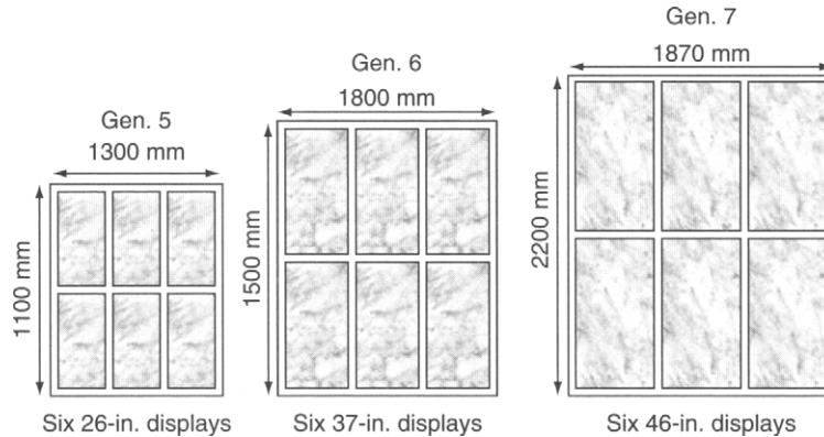
Figure 3.31: Optimized TV display sizes on different-sized substrates.
