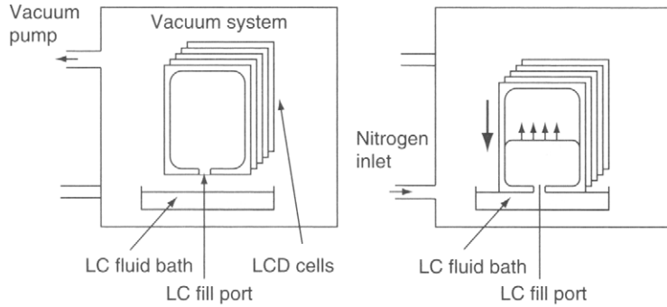
Figure 3.22: Filling of LC cells through fill ports by nitrogen backfill in a vacuum system.
