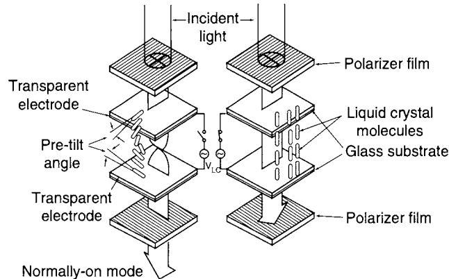
Figure 1.10: Operation of twisted nematic (TN) LC cell.
