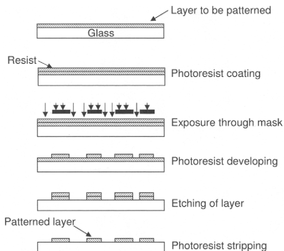
Figure 3.6: Photolithography sequence.
