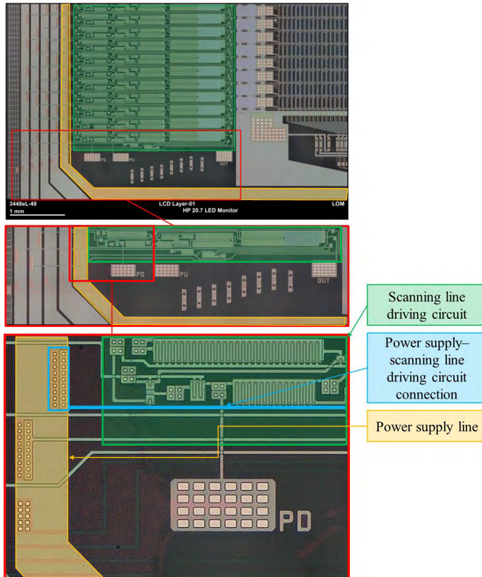
LOM: LCD Layer, bottom left (1mm)
