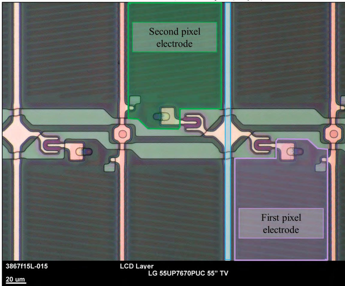
LG 55" UP7670PUC, LCD Layer (20 \mu\text{m} )
