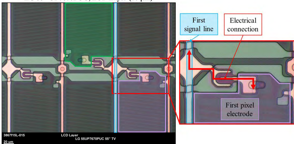
LG 55" UP7670PUC, LCD Layer (20 \mu\text{m} )
