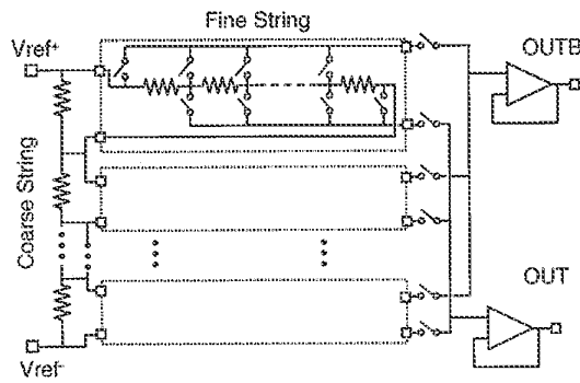
Fig. 13. Dual resistor string DAC schematic.
