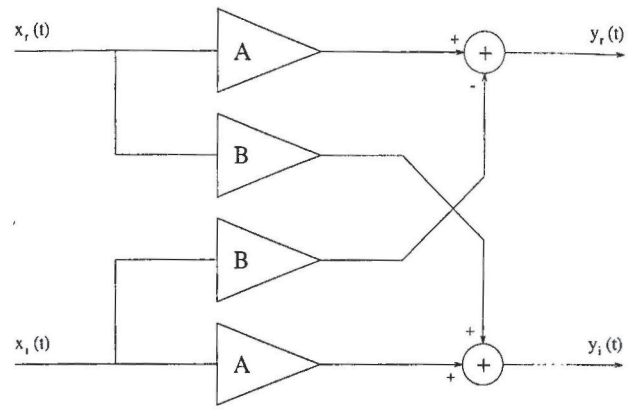
Fig. 7. Block scheme of the amplification of a complex signal with a complex constant.
