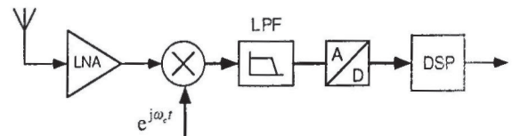
Fig. 20. The zero-IF receiver topology in compact notation.
