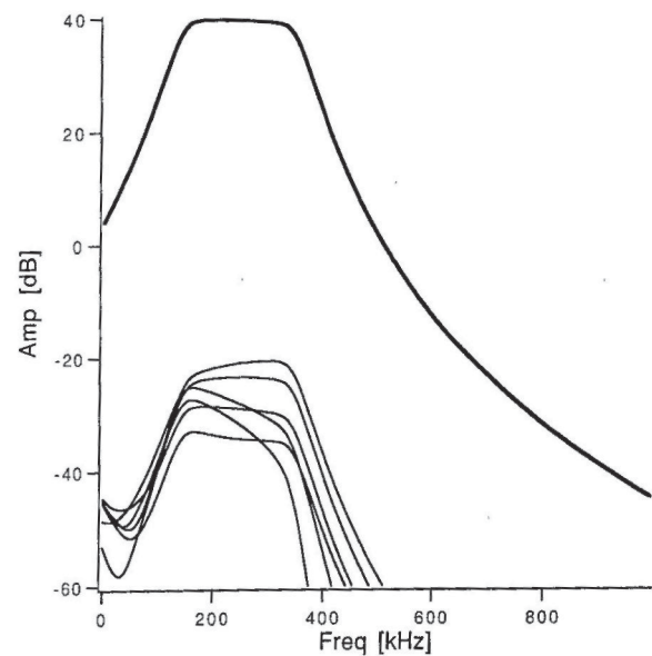
Fig. 18. Monte Carlo simulation of the signal crosstalk from negative to positive frequencies for the translated fifth-order Butterworth filter.
