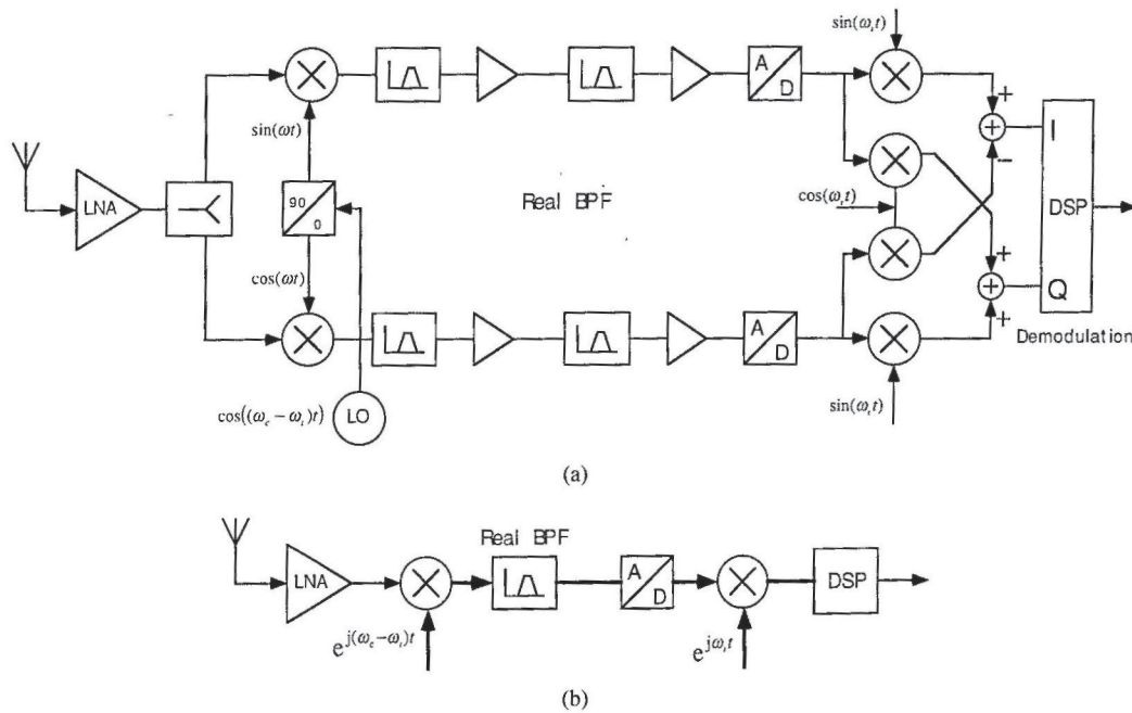
Fig. 22. The topology of a low-IF receiver which uses real filters in the LF part. (a) Full notation and (b) compact notation.
