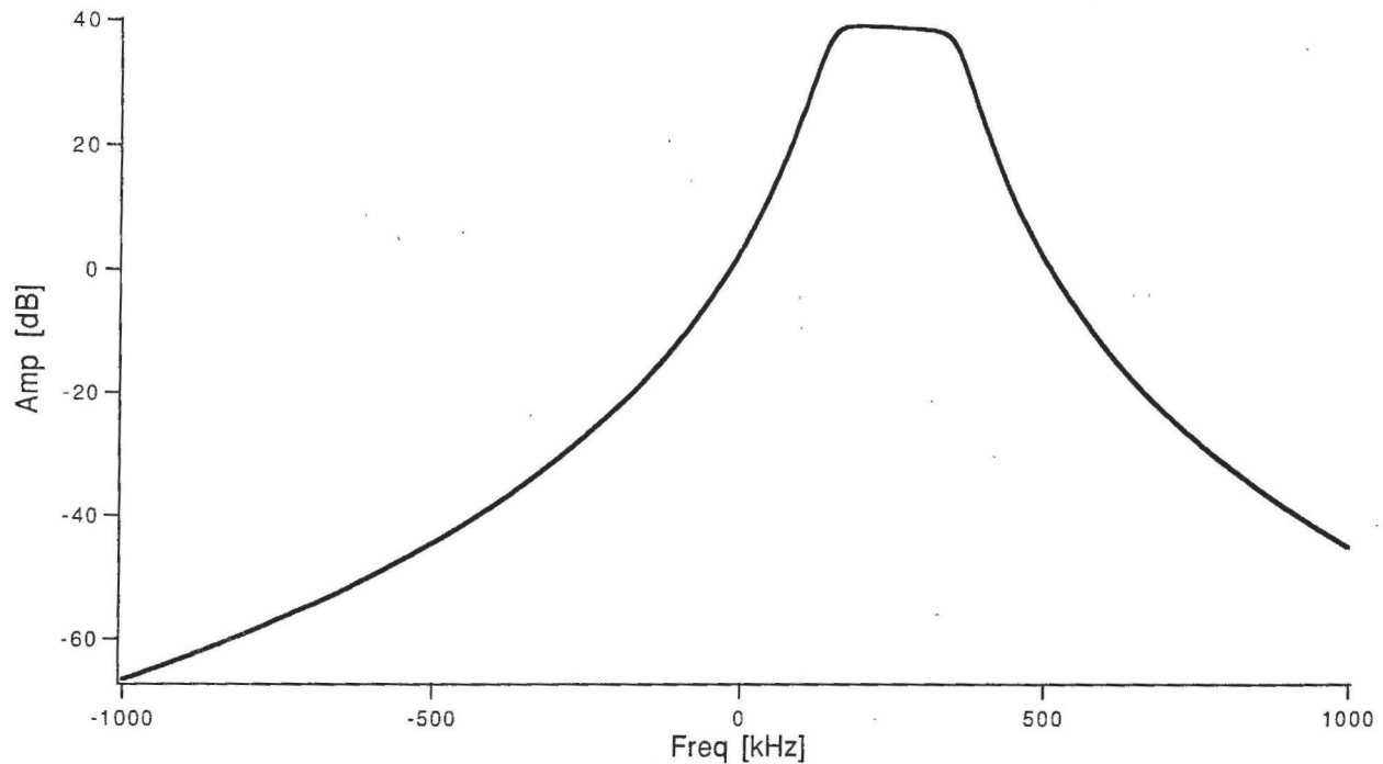
Fig. 17. Transfer function of a frequency translated fifth-order low-pass Butterworth filter.
