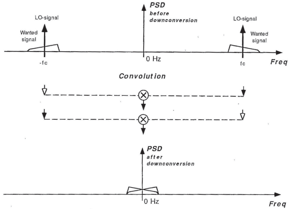
Fig. 4. Direct downconversion by mixing the RF signal with a single sine.
