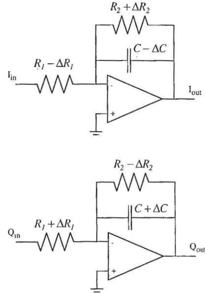
Fig. 11. Mismatch in a low-pass filter for complex signals.
