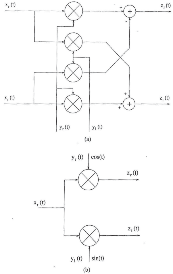
Fig. 8. (a) The multiplication of a complex signal with a complex signal. (b) The special case of the multiplication of a real signal with a complex signal.
