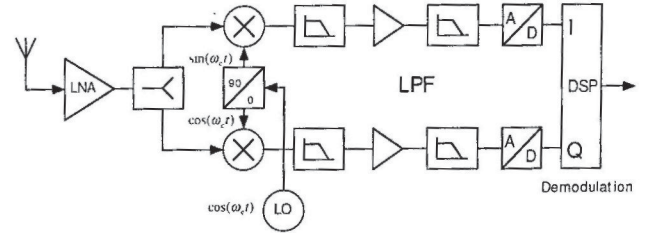
Fig. 5. The zero-IF receiver topology.
