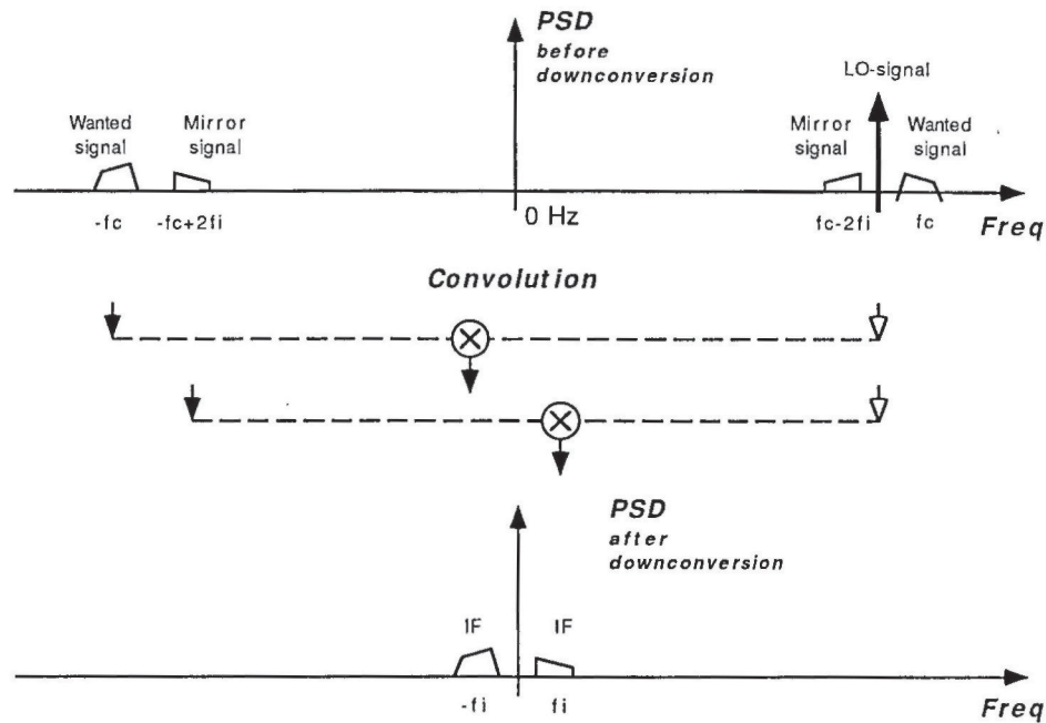
Fig. 19. Downconversion to a low IF.
