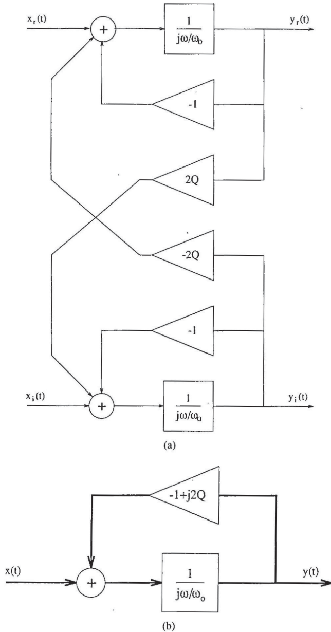
Fig. 15. Block scheme for the realization of a single complex pole. (a) The full notation and (b) the compact notation.
