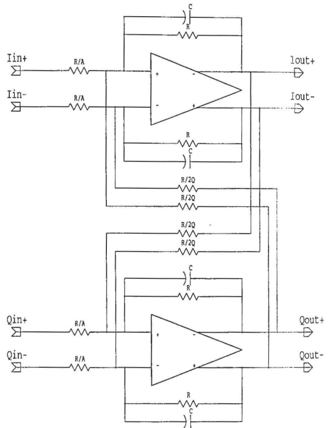
Fig. 16. Realization of a single complex pole with the active- RC filter technique.
