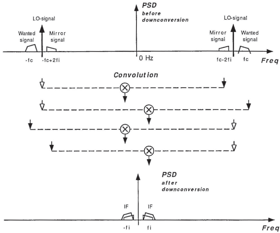
Fig. 2. The downconversion scheme in an IF receiver.
