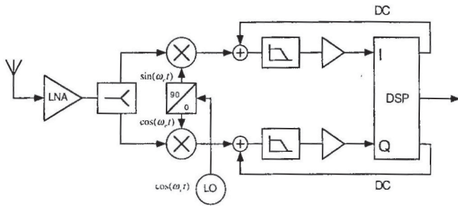
Fig. 6. A zero-IF receiver with a DC compensation feedback path.
