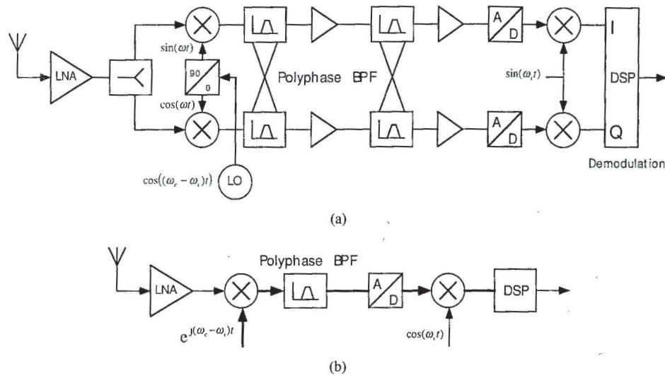
Fig. 21. The topology of a low-IF receiver which uses a complex bandpass filter in the LF part. (a) Full notation and (b) compact notation.
