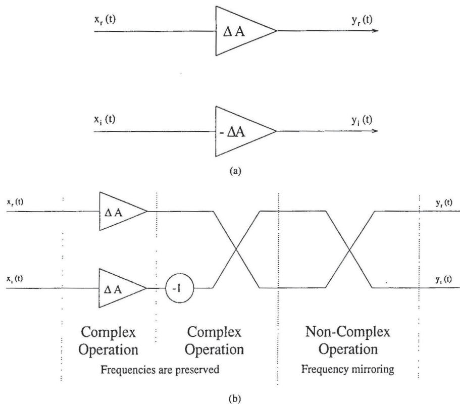
Fig. 10. (a) Mismatch between the amplification in the real and imaginary path. (b) Equivalent scheme.
