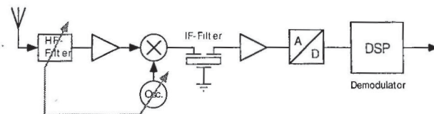
Fig. 1. Schematic representation of the IF receiver topology.
