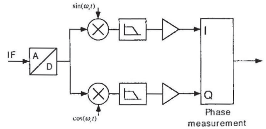
Fig. 3. Demodulation with a DSP of a signal situated on an IF.
