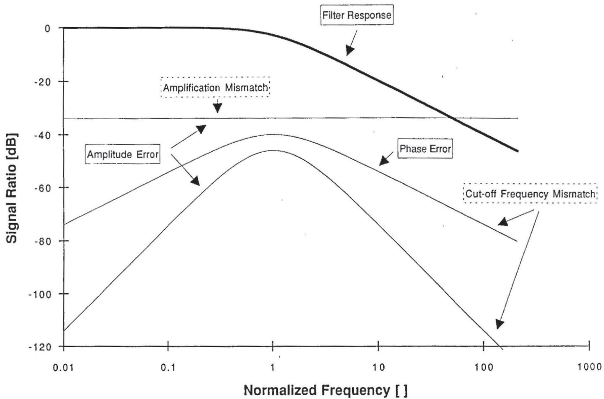
Fig. 12. Signal mirroring caused by mismatch in a low-pass filter for complex signals in function of frequency.
