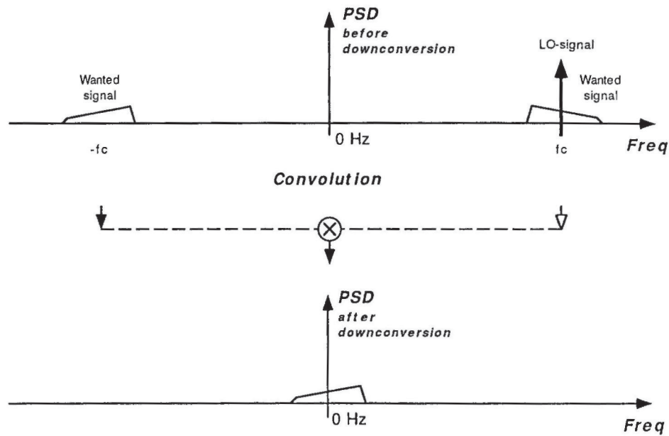
Fig. 9. Downconversion in a zero-IF receiver: mixing with a positive frequency.
