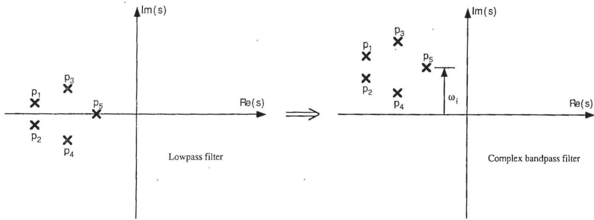
Fig. 13. S -plane representation of the frequency translation of a fifth-order low-pass filter.
