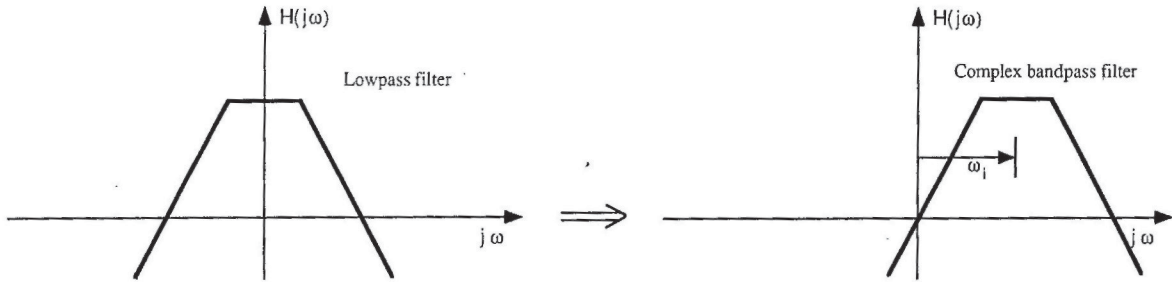
Fig. 14. The effect of a frequency translation on the transfer function.
