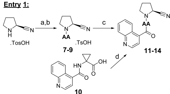
Scheme 1. Synthesis of P2-Modified FAP Inhibitors 11–14 and 16–27 a
