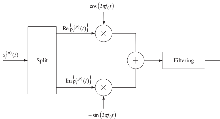
Figure 6.13-1: Downlink modulation
