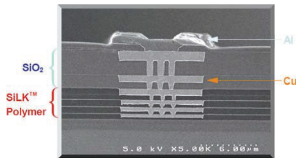
Fig. 2.23 Scanning electron micrograph of IBM's 130 nm Cu-damascene process with SiLK polymer (Reproduced with permission, IBM Research)
