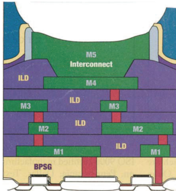
Fig. 2.7 Multilayer metallization with interlayer dielectric (ILD) (Reprinted with permission, Air Products and Chemicals, Inc., 2002)
