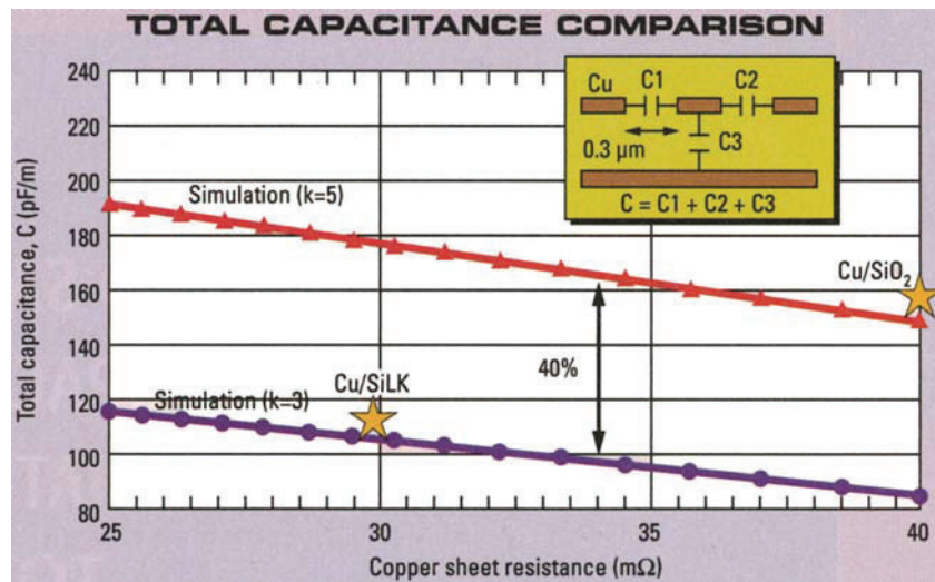
Fig. 2.10 The effective capacitance effect of low- K on Cu-interconnects (Reprinted with permission, Semiconductor International, June 2000, p. 118)
