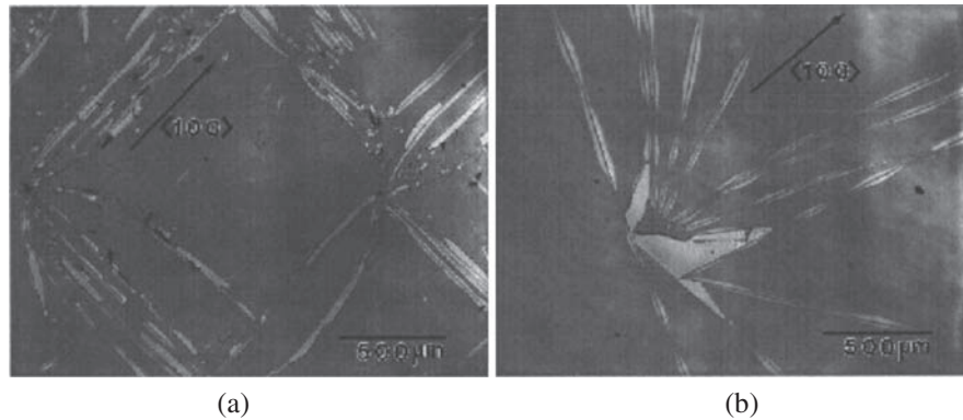
Fig. 2.17 (a) Xerogel cracking on a <100> Si-wafer, and (b) cracking on a <111> silicon wafer (Photo courtesy, Prof. K.N. Tu, UCLA, CA)
