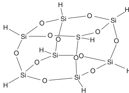
Fig. 2.25 Another form of hydrogen silsesquioxane (HSQ) which resembles a cage structure
