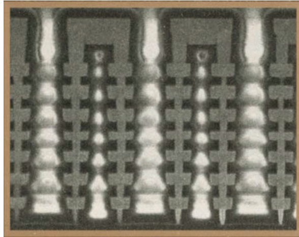
Fig. 2.19 Eight-level Cu/black diamond integration (Reprinted with permission, Applied Materials)
