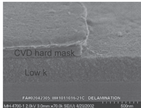
Fig. 2.13 Typical cap delamination failure (Reproduced with permission, AMD)
