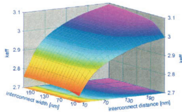
Fig. 2.12 Simulated results for the effect of variation of geometrical dimensions on K_{\text{eff}} (Photo courtesy, Prof. T. Gessner, Chemnitz University of Technology)
