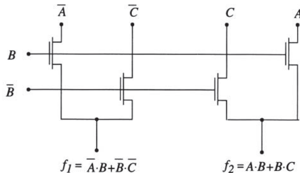
Figure 9.35 General logic arrangement in CPL
