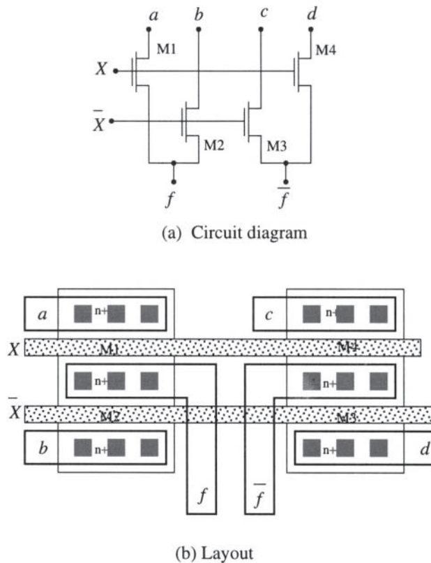
Figure 9.36 2-input array layout example
