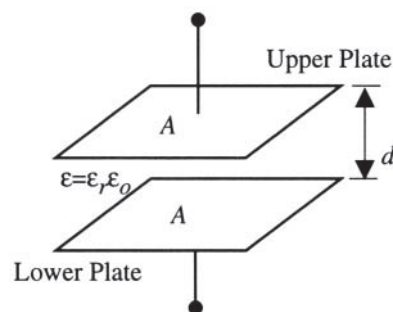
Figure 7.27 Parallel-plate capacitor
