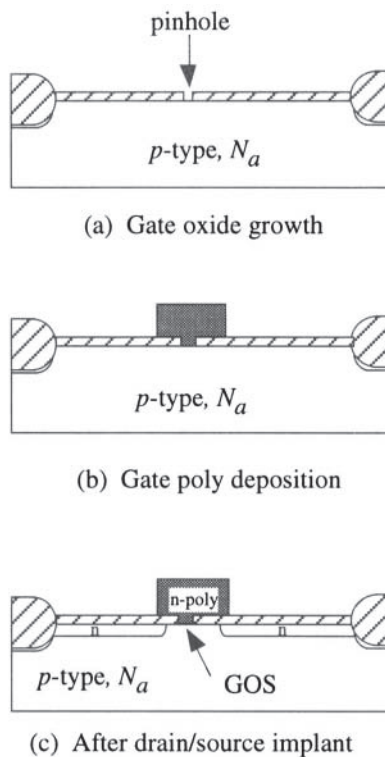
Figure 2.43 Gate-oxide shorts in MOSFETs
