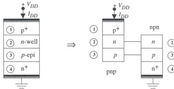
Figure 2.36 4-layer modelling of the latchup network
