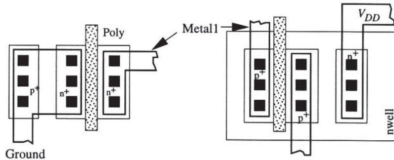
Figure 2.27 Metal1 patterning
