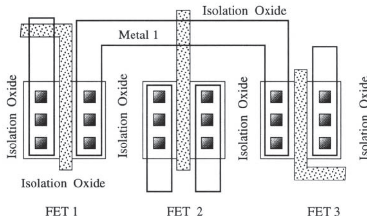
Figure 2.12 Use of isolation oxides to electrically separate FETs
