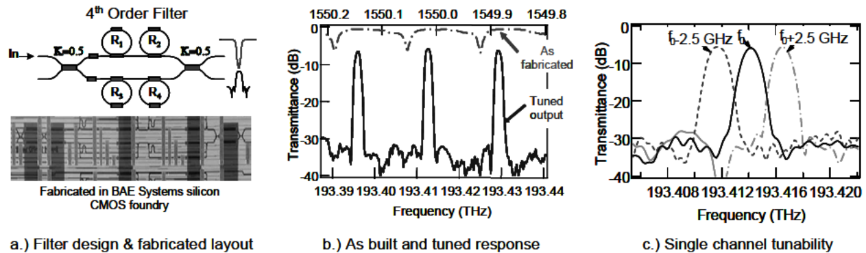
Fig. 5. 4 th order zero pole filters using TE mode silicon waveguides a.) 4 th order filter schematic and fabricated chip, b.) as fabricated and tuned filter response showing narrow 3dB bandwidth of 1.0GHz and stopband rejection of 25dB, c.) wide channel frequency tuning of \pm 2.5 GHz with no loss in filter shape
