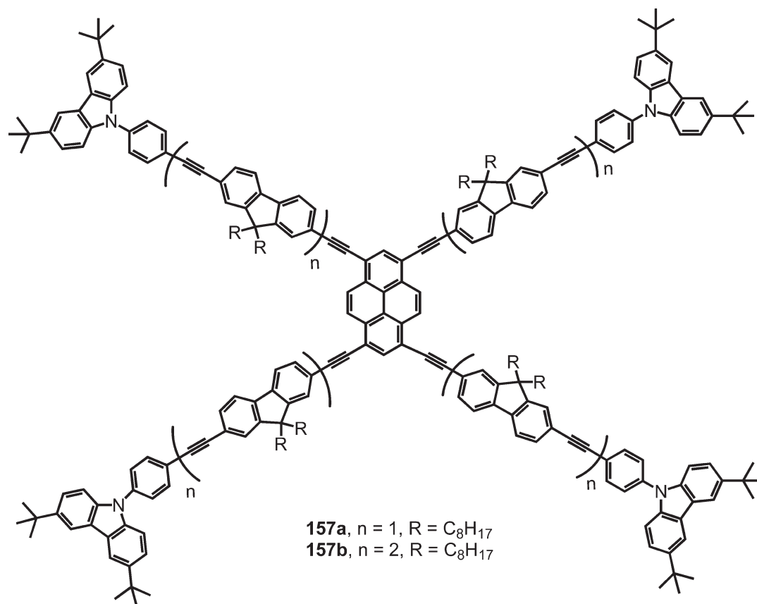
Figure 84. First-generation carbazole/fluorene dendrimer with pyrene at the core (157).
