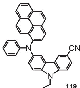
Figure 55. Chemical structure of 3-cyano-9-diarylamino carbazole 119.
