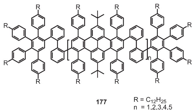
Figure 101. Graphitic nanoribbons 177.
