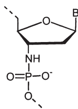
N3'-P5' Phosphoroamidate (NP)
