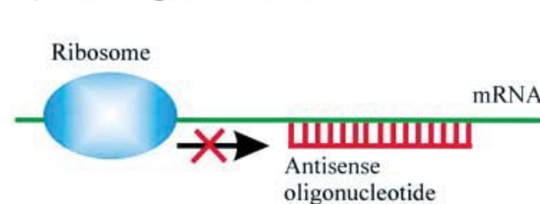
Fig. 2. Mechanisms of antisense activity. (A) RNase H cleavage induced by (chimeric) antisense-oligonucleotides. (B) Translational arrest by blocking the ribosome. See the text for details.
