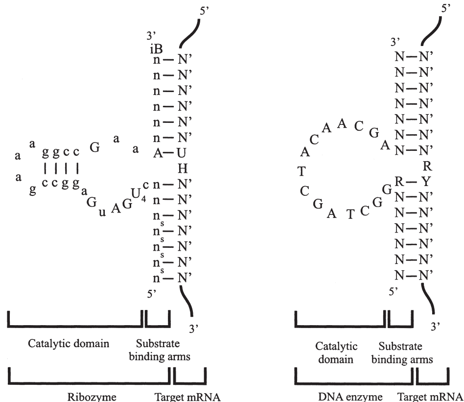
Fig. 5. Secondary structure models for the hammerhead ribozyme and the 10-23 DNA enzyme. A nuclease-resistant ribozyme according to Usman and Blatt [111] is shown. It consists of 2'- O -methyl RNA (lower case), five ribonucleotides (upper case), a 2'- C -allyluridin at position 4, four phosphorothioate linkages (s) and an inverted 3'-3' deoxabasic sugar. The DNA enzyme shown consists entirely of DNA nucleotides; R is a purine, Y is a pyrimidine.
