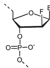
2'-fluoro-arabino nucleic acid (FANA)
