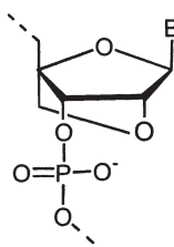
Locked nucleic acid (LNA)
