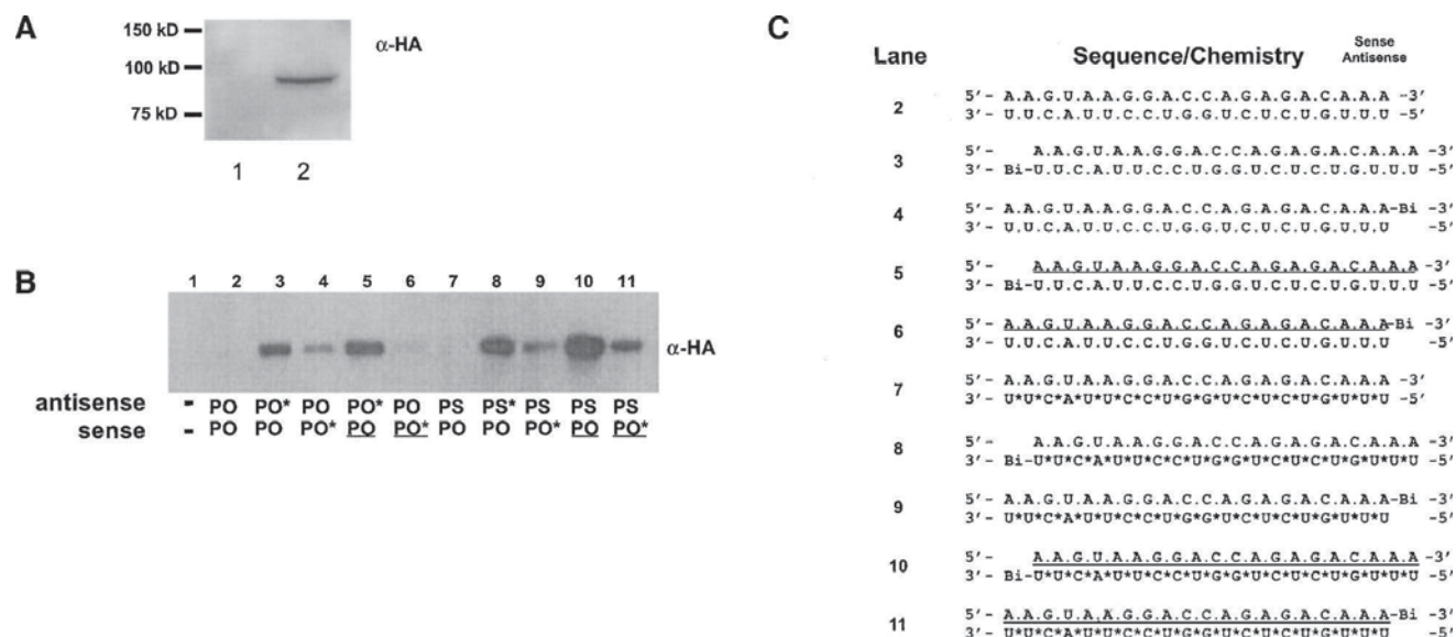
FIGURE 5. Modified siRNAs interact with overexpressed hAgo2. (A) Characterization of pE2-N H A. Total HeLa lysates prepared from untreated cells (lane 1) and cells expressing HA-hAgo2 (lane 2) were separated by SDS-PAGE and immunoblotted with anti-HA antibodies. The migration of the molecular mass standards is shown on the left. (B) Western blot analysis of biotin-siRNA samples isolated from HeLa cells expressing HA-hAgo2. Biotin-tagged strands were isolated from total cell lysates, as described in Materials and Methods. Isolates were then subjected to SDS-PAGE and Western blotted with anti-HA antibody. (C) Structure and sequence of siRNA constructs included in analysis. (*) A PS modification, (underline) 2'-OMe-modified nucleotides, (Bi) biotin residue.
