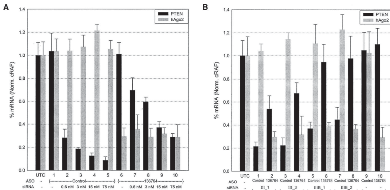
FIGURE 4. Modified siRNA activity is attenuated by knock-down of hAgo2. (A) Validation of ASO knock-down assay in HeLa cells. siRNA (I_1) was transfected into HeLa cells at a dose of 0.6–75 nM post-treatment with either the control ASO (ISIS 129686) or the ASO specific for hAgo2 (ISIS 136764). (B) Effect of hAgo2 knock-down on activity of siRNAs containing a full 2'-OMe-modified sense strand. Modified and unmodified siRNAs targeting PTEN Site III were transfected (75 nM) into HeLa cells previously treated with ISIS 129686 or ISIS 136764. PTEN and hAgo2 mRNA levels were determined relative to the cRAF mRNA level by real-time RT-PCR (TaqMan). The results shown represent the percentage of untreated control expression (UTC). Each bar represents the mean of three biological replicates ( \pm standard deviation). The control ASO (ISIS 129686) is a random sequence that has no significant homology to the human genome.
