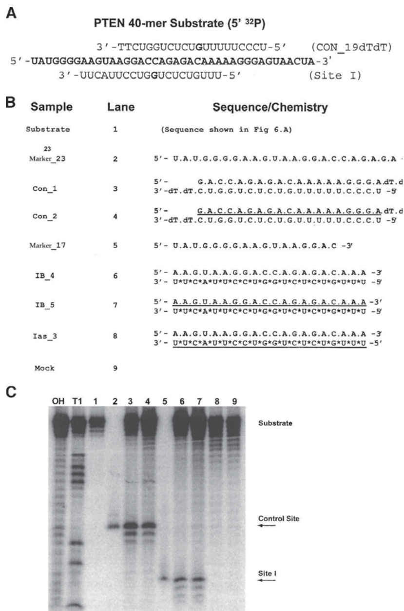
FIGURE 7. Modified siRNAs enter into the hAgo2/RISC complex to mediate target RNA cleavage. (A) A 5'-[P32] end-labeled 40-mer substrate containing Site I was incubated with immunopurified RISC complexes, as described in Materials and Methods. The sequence of siRNA constructs and lane assignments are shown in B. The sequence of each RNA marker corresponds to the expected cleavage product of 23 nt (control site) or 17 nt (Site I). (*) A phosphorothioate modification, (underline) 2'-OMe-modified nucleotides. (C) Cleavage products were resolved on a 12% polyacrylamide 7 M urea gel. The 5' cleavage products are indicated by arrows. Sequence identity was assigned according to the control digestions of the substrate by RNase T1, base (OH) hydrolysis, and synthetic RNA markers.
