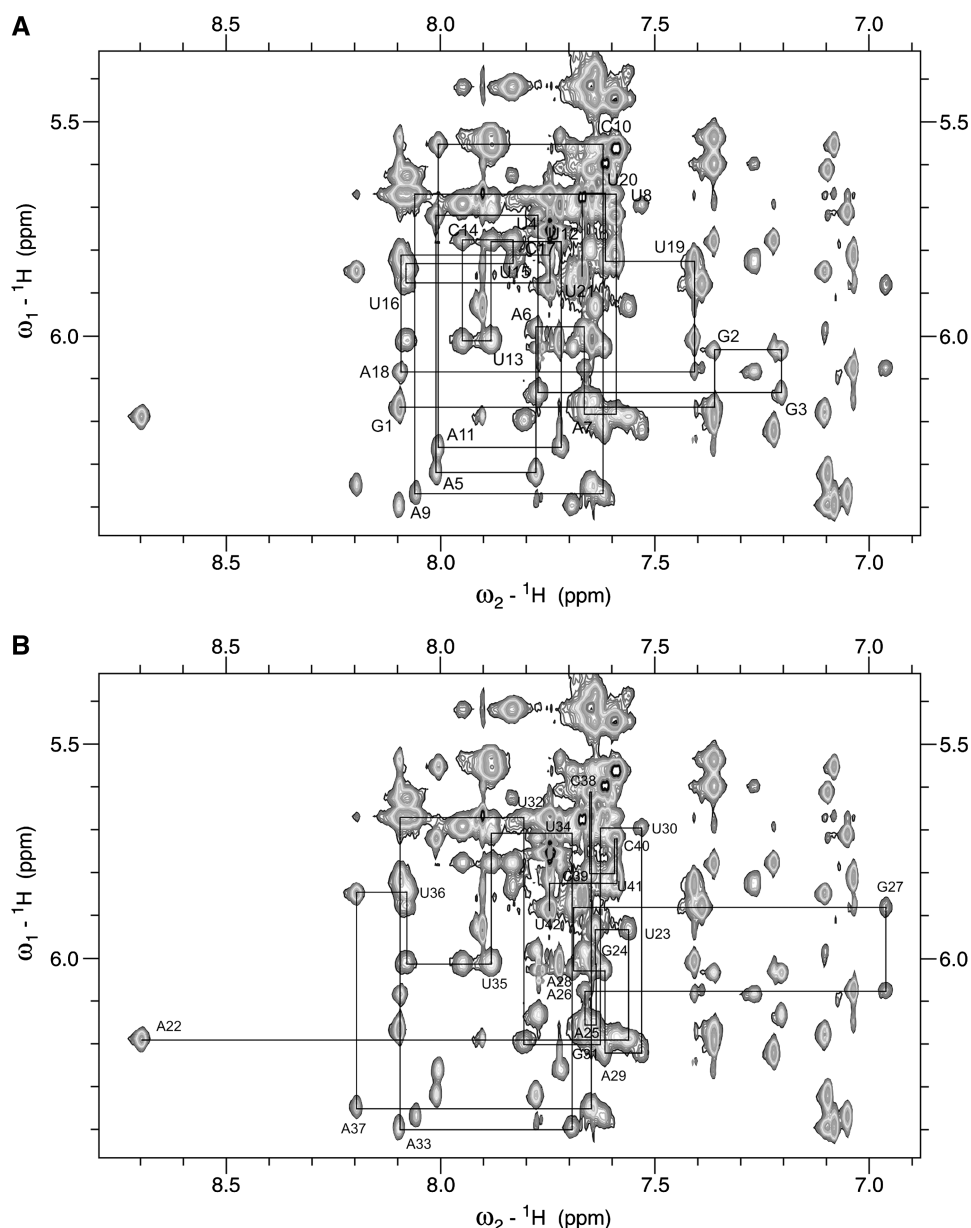
Figure 6. The aromatic–anomeric region of the 2D NOESY spectrum ( \tau_m = 150 ms, 25^\circ\text{C} ). Lines represent the sequential walk for the sense, G1–U21 ( A ) and antisense, A22–U42 ( B ) strands, which are shown separately to reduce overlap.
