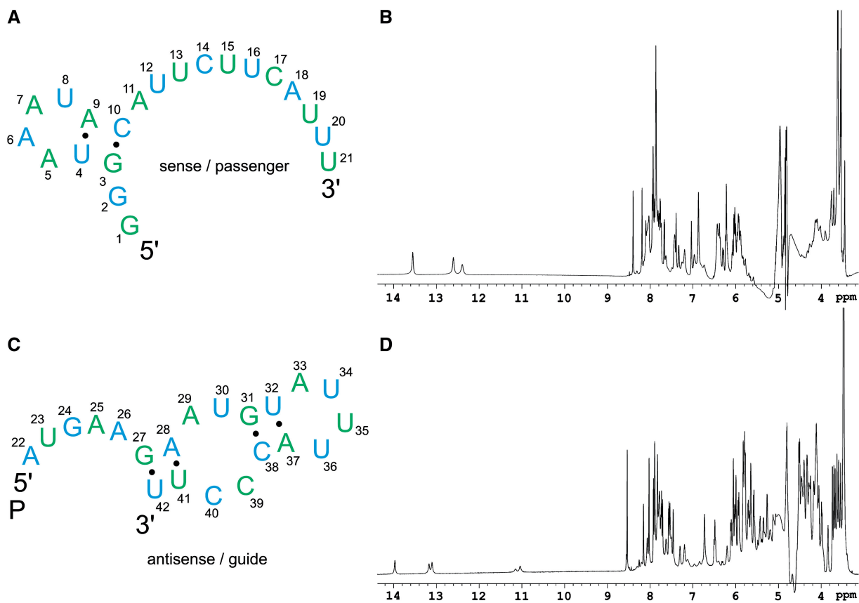
Figure 3. Base pairing pattern of the sense (A) and antisense (C) strands and the corresponding 1D ^1\text{H} NMR spectra of individual sense (B) and antisense (D) strands recorded at 15°C.
