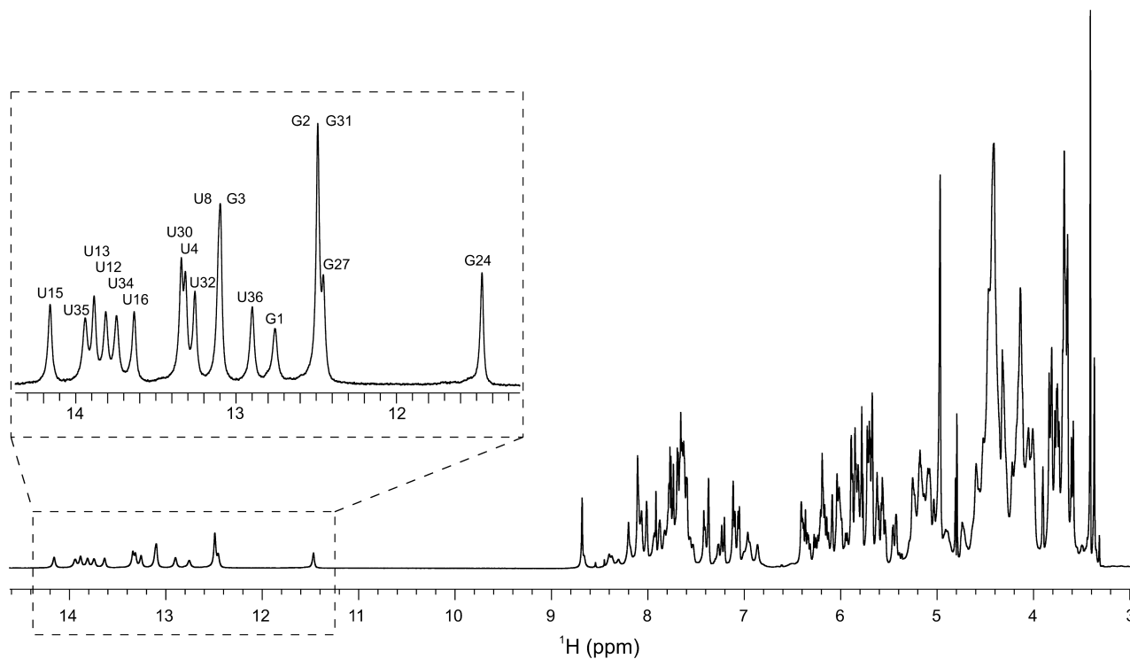
Figure 4. 1D ^1\text{H} NMR spectrum of the dimeric RNA construct recorded at 25°C. Imino region with the assignment of resonances is shown in the inset.
