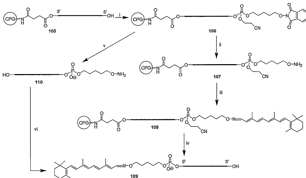
Scheme C: Conjugation of all- trans -retinal to oligonucleotides
