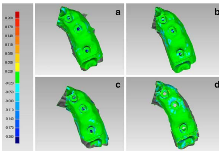
Fig. 5 Precision in the partially edentulous maxilla, occlusal view. The best single result obtained with each device were: (a) CS 3600® 19 \pm 50 \mu\text{m} ; (b) Trios 3® 21 \pm 42 \mu\text{m} ; (c) Cerec Omnicam® 25 \pm 53 \mu\text{m} ; (d) True Definition® 15 \pm 28 \mu\text{m}
