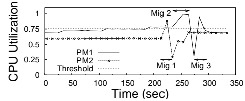
Figure 4: After a hotspot is detected on PM_1 , a swap occurs via the scratch PM. Initially, VM_1 and VM_2 are on PM_1 . VM_2 is swapped with VM_4 from PM_2 to resolve overload.
