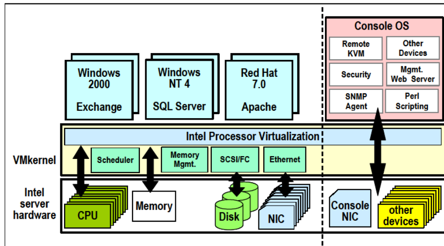
Figure 2-7 VMware ESX Server architecture with Console OS
