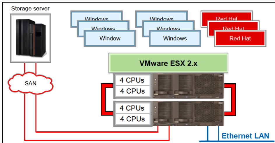
Figure 3-6 16-way x445 running a single system image
