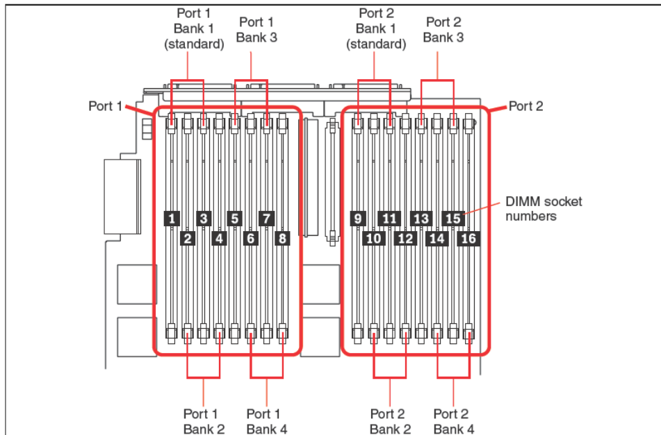
Figure 3-5 Memory DIMM sockets on the x445 SMP Expansion Module
