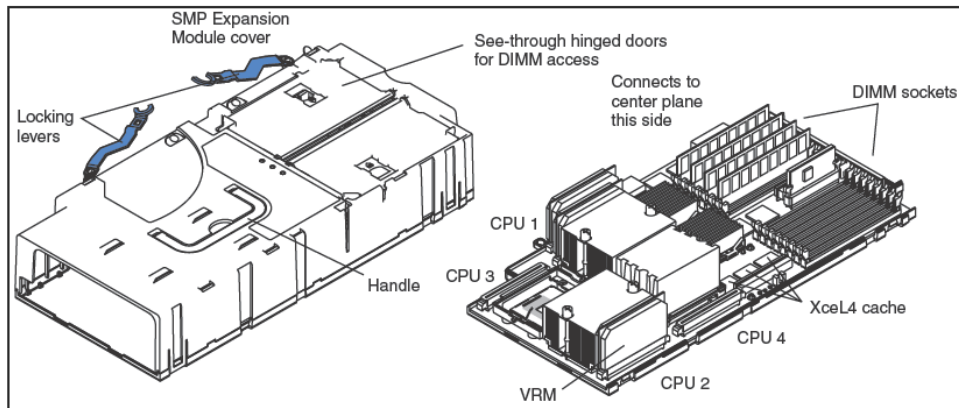
Figure 3-4 xSeries 445 SMP Expansion Module
