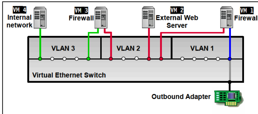
Figure 2-6 Using VLANs to create a DMZ
