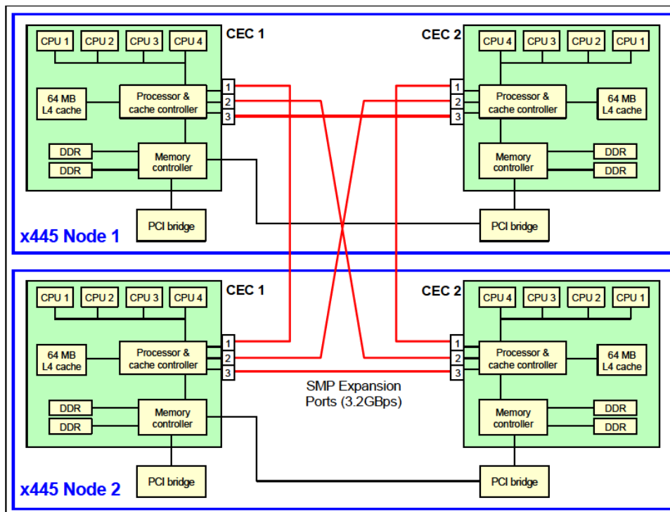
Figure 3-2 Two 8-way x445 servers connected as a 16-way configuration
