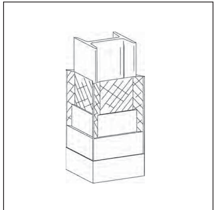
Figure 7 Column Protection - Metal Lath and Plaster
