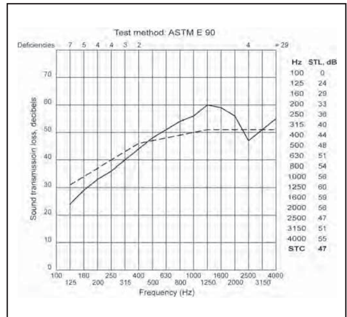
Figure 10 STL Curve
