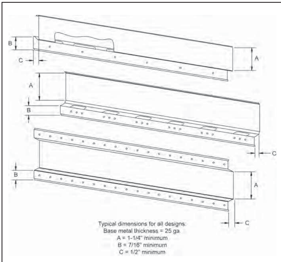
Figure 8 Typical Resilient Furring Channels
