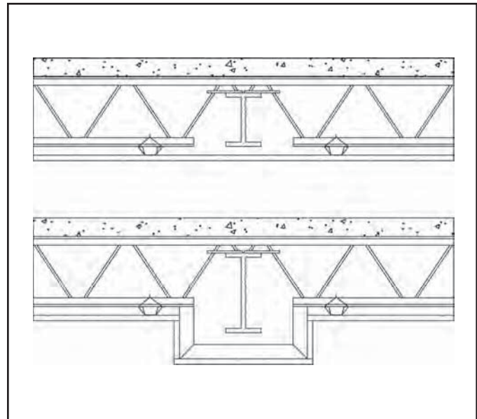
Figure 4 Membrane Protected Steel Beam- Continuous
