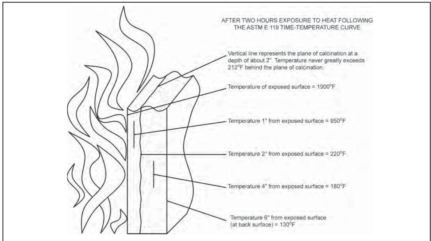
Figure 1 How Gypsum Retards Heat Transmission
