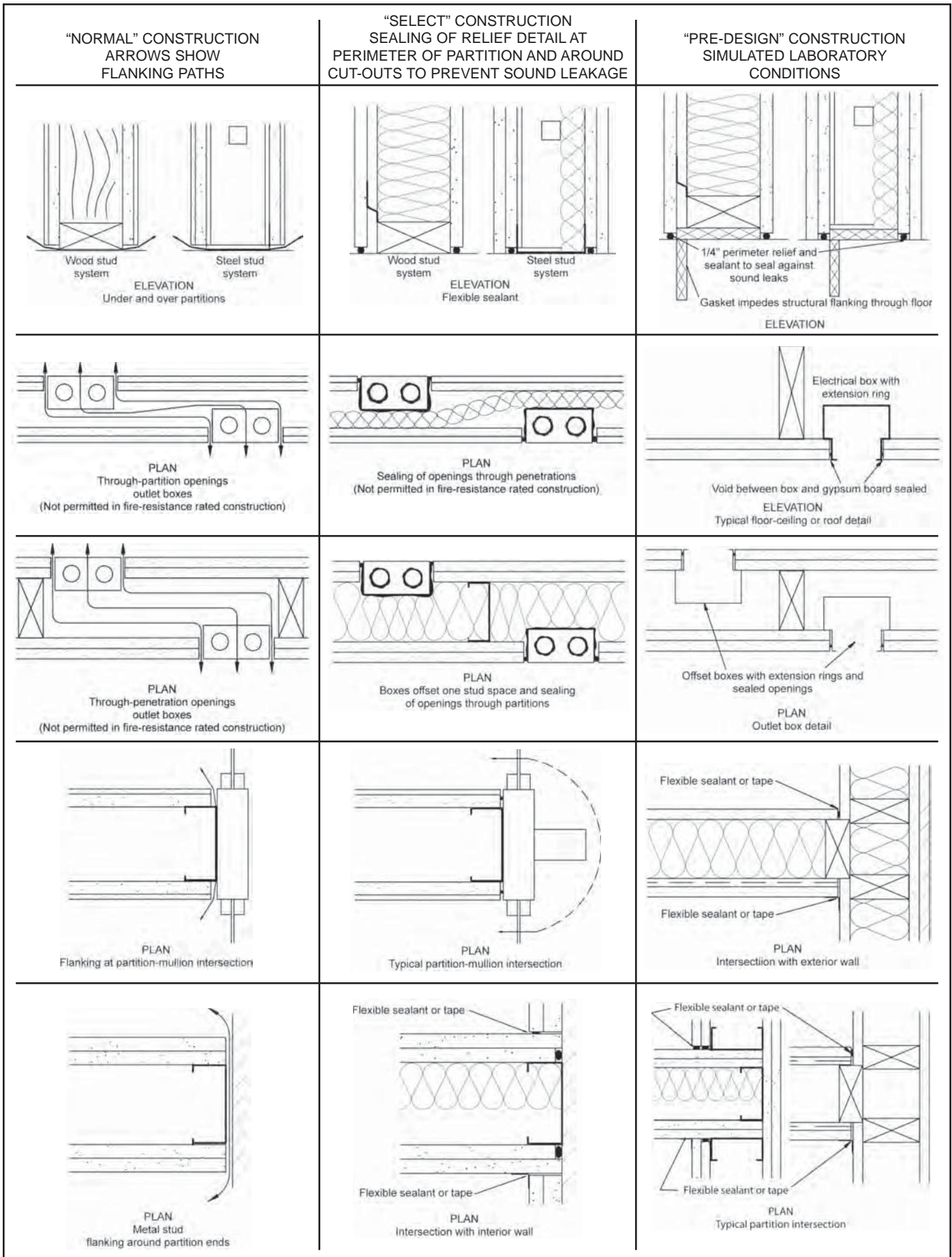
Figure 9 Sound Isolation Construction
