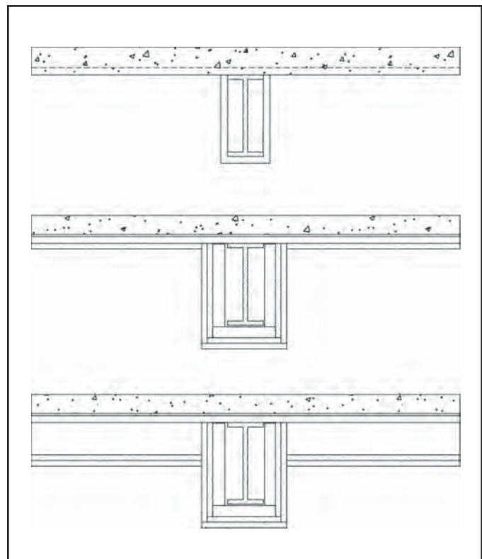
Figure 5 Steel Beam - Individual Encasement Protection
