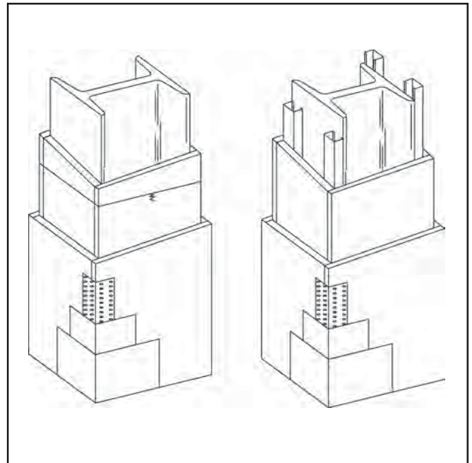
Figure 6 Column Protection - Gypsum Panel Product
