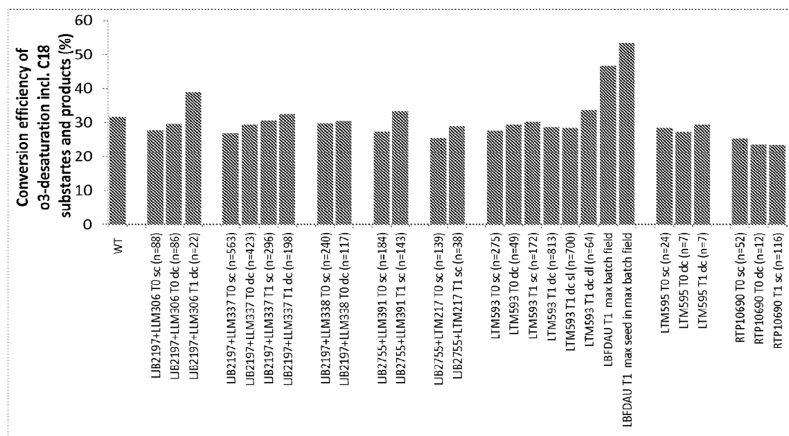
Figure 37: Conversion efficiencies of omega-3 desaturation (including C18 fatty acids) in seed of transgenic Brassica napus and in Brassica napus wildtype seeds. See caption in Figure 32 for further details.
