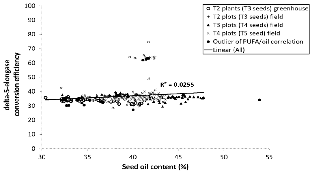
Figure 64: The conversion efficiency of the delta-5-elongase was not correlated with seed oil content. Shown are data of 3 generations of event LANPMZ. For the greenhouse data, one marker corresponds one seedbatch of one plant, for the field data, one marker corresponds to an analysis on a random selection of seeds representing one plot.
