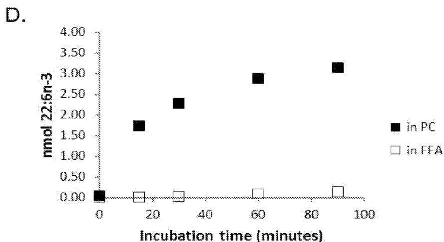
Figure 26: Examples of Desaturase Enzyme Reactions Showing Specificity for Acyl-lipid substrates. [ 14 C]Fatty acid methyl esters (ME's) were isolated from the enzymatic reactions containing microsomes obtained from a yeast strain expressing the protein of interest, resolved by TLC as described for each specific enzyme and detected by electronic autoradiography using Instant Imager. In panel A Delta-12 Desaturase (Ps), c-d12Des(Ps_GA), desaturated enzyme products were only detected in the phosphatidylcholine fraction indicating the enzyme was specific for an acyl-lipid substrate. In panel B and panel C Delta-4 Desaturase (Tc), c-d4Des(Tc_GA), desaturated enzyme products were detected in the phosphatidylcholine fraction indicating the enzyme was specific for an acyl-lipid substrate. In panel D was a time-course demonstrates of the Delta-4 Desaturase (Tc), c-d4Des(Tc_GA).
