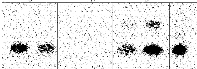
Figure 29: Examples of Elongase Activity in transgenic Brassica napus . [ ^{14}\text{C} ]Fatty acid methyl esters (ME's) were isolated from the enzymatic reactions, resolved by TLC as described for each specific enzyme and detected by electronic autoradiography using Instant Imager. In panel A Delta-6 Elongase, activity was demonstrated by comparison of enzyme activity from yeast microsomes isolated from a strain expressing the d6E(Pp protein relative to microsomes isolated from transgenic B. Napus containing the d6Elo (Pp_GA2) gene and the d6Elo (Tp_GA2). In panel B the Delta-5 Elongase (Ot), c-d5Elo(Ot_GA3), activity was demonstrated by comparison of enzyme activity from yeast microsomes isolated from a strain expressing the c-d5Elo(Ot_GA3) protein relative to microsomes isolated from transgenic B. Napus containing the d5Elo (Ot_GA3) and a wild-type B. napus (control).
