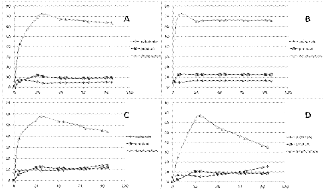
Figure 30: Time course optimization. Yeast cells expressing the c-d5Des(Tc_GA2) were fed with 0.25 mM HGLA and the production of ARA was determined by GC. Samples were collected starting immediately after feeding. In Panels A-D, Desaturation was represented as %Conversion vs Growth Time (hours) and Product and Substrate levels are represented as %Total Fatty acid vs Growth time (hours). Panel A Samples supplied with HGLA immediately after induction. Panel B overnight induction (22hrs) before feeding. Panel C cultures supplied with 3X normal HGLA level Panel D. cultures supplied with normal rate of HGLA (0.25 mM) daily.
