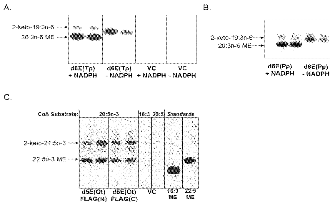
Figure 28: Examples of Elongase Enzyme Activity Heterologously Expressed in Yeast. [ ^{14}\text{C} ]Fatty acid methyl esters (ME's) were isolated from the enzymatic reactions, resolved by TLC as described for each specific enzyme and detected by electronic autoradiography using Instant Imager. All FAME's shown had similar R_f 's as authentic standards. In the absence of [ ^{14}\text{C} ]malonyl-CoA no radioactive fatty acids were observed in any of these elongase reactions. In panel A delta-6 elongase (Tp), c-d6Elo(Tp_GA2), activity was demonstrated by comparison of enzyme activity present in yeast microsomes isolated from a strain expressing the c-d6Elo(Tp_GA2) protein relative to microsomes isolated from a control strain containing an empty vector (VC). In panel B, delta-6 elongase (Pp), c-d6Elo(Pp_GA2), was demonstrated by comparison of enzyme activity from yeast microsomes isolated from a strains expressing c-d6Elo(Pp_GA2) protein to microsomes isolated from a control strain containing an empty vector (VC), as shown in panel
