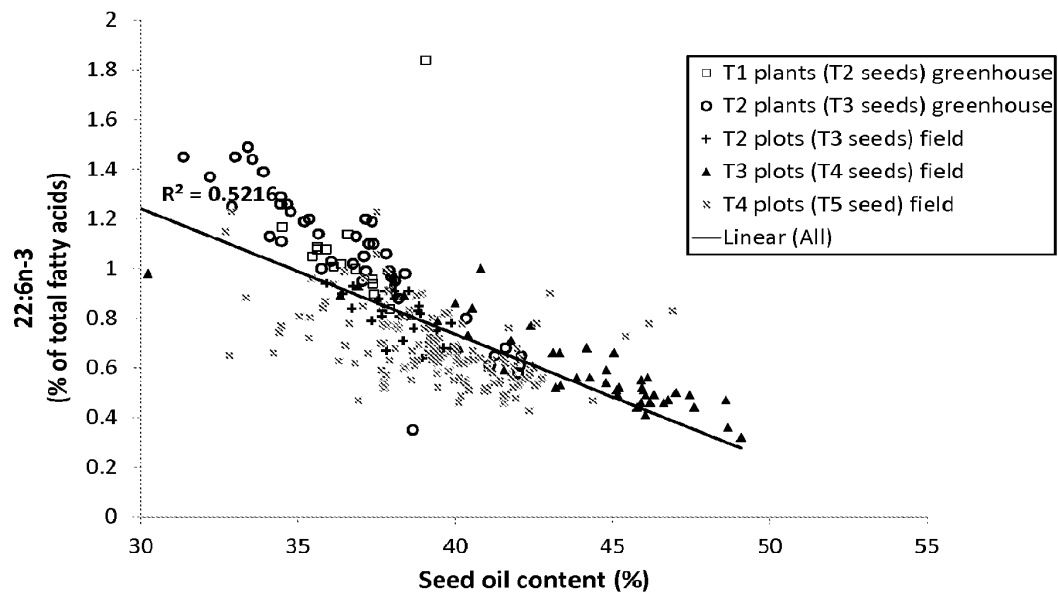
Figure 78: The total fatty acid percentage of 22:6n-3 (DHA ) correlated with seed oil content. Shown are data of 4 generations of event LAODDN. For the greenhouse data, one marker corresponds one seedbatch of one plant, for the field data, one marker corresponds to an analysis on a random selection of seeds representing one plot.
