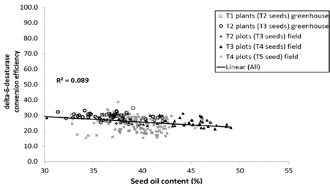
Figure 49: The conversion efficiency of the delta-6-desaturase was negatively correlated with seed oil content. Shown are data of 4 generations of event LAODDN. For the greenhouse data, one marker corresponds one seedbatch of one plant, for the field data, one marker corresponds to an analysis on a random selection of seeds representing one plot.
