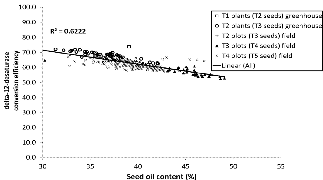
Figure 45: The conversion efficiency of the delta-12-desaturase was negatively correlated with seed oil content. Shown are data of 4 generations of event LAODDN. For the greenhouse data, one marker corresponds to one seed batch of one plant, for the field data, one marker corresponds to an analysis on a random selection of seeds representing one plot.
