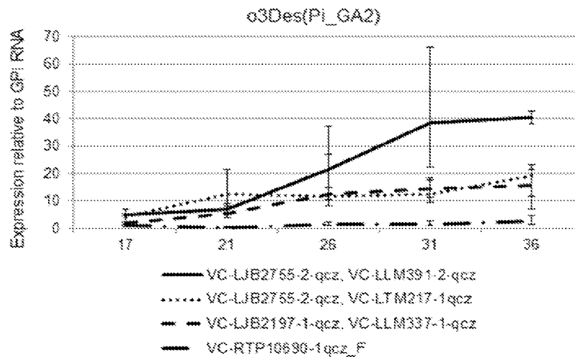
Figure 16: Comparative transcript analysis o3Des(Pi_GA2) driven by the VfUSP promoter during seed development of single copy event of four different construct combinations.
