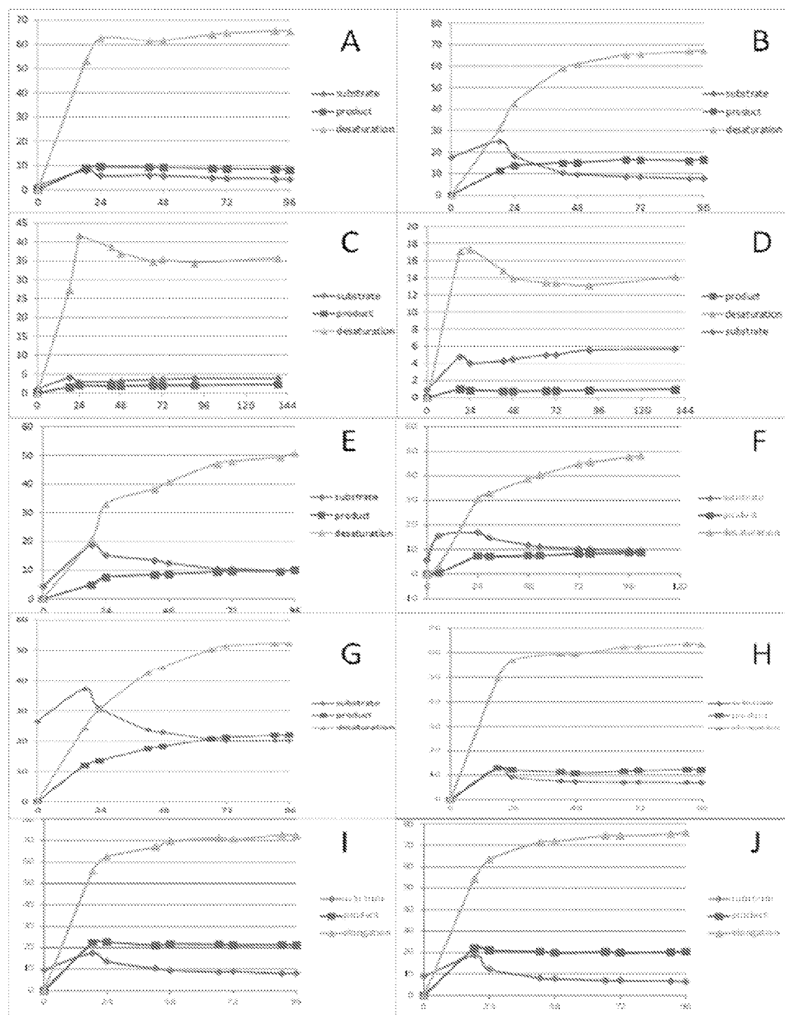
Figure 31: Representative time course graphs for all desaturases and elongases. Yeast cells expressing each enzyme were supplied with 0.25 mM of preferred fatty acid substrate, and fatty acid profiles were obtained by GC at
