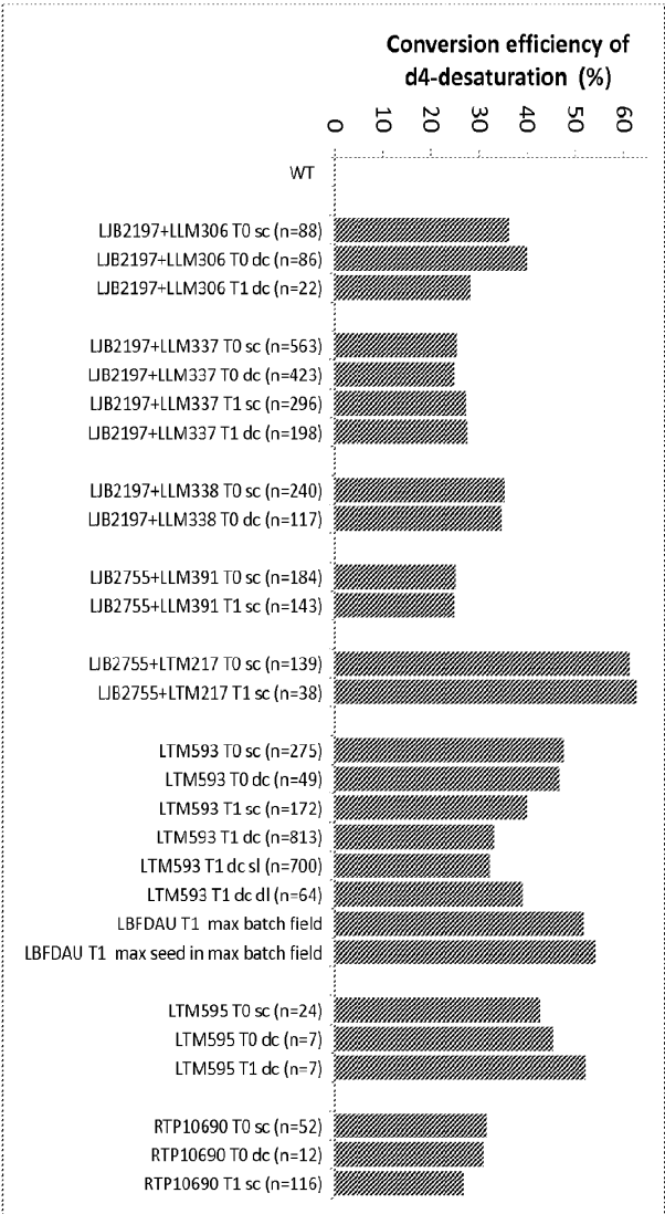
Figure 39: Conversion efficiencies of delta-4-desaturation in seed of transgenic Brassica napus and in Brassica napus wildtype seeds. See caption in Figure 32 for further details.
