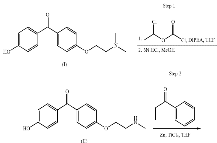
Schema 1. Synthesis of (Z)-endoxifen Free Base
