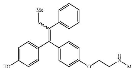
Formula (III)
